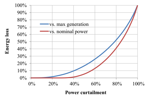
Fig. 4. Lost energy as a function of curtailed power in a Finnish PV system. Power curtailment percentage is calculated in relation to nominal power (red curve) and maximum generated power (blue). (For interpretation of the references to color in this figure legend, the reader is referred to the web version of this article.)
