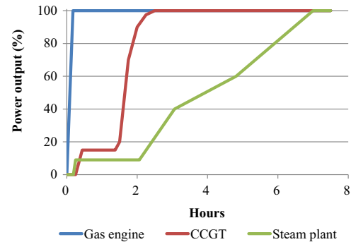
Fig. 3. Start-up and ramp-up times of three technologies after a five-days stop [68].
