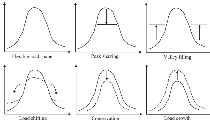
Fig. 1. Categories of demand side management [30].
