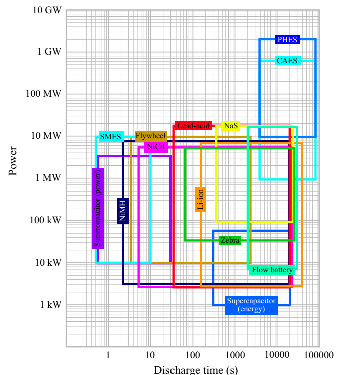
Fig. 2. Power and discharge time of selected energy storage technologies [250,392,393].
