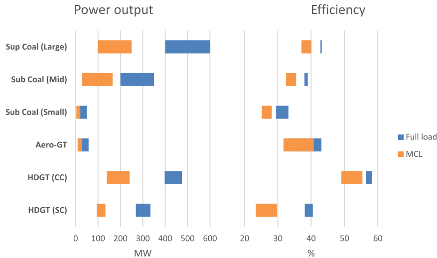
Fig. 8. Comparison of the power output and efficiency at full load and minimum complaint load (MCL) for the different technologies.
