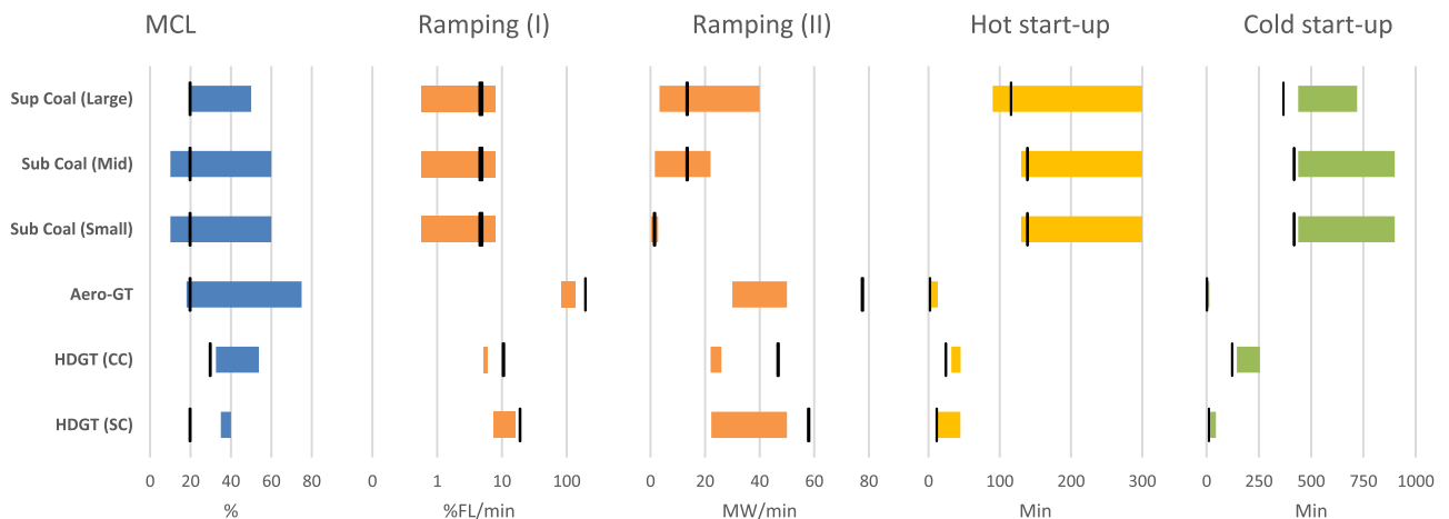
Fig. 10. Comparison of different flexibility processes for the different technologies. Black bars represent possible future values.
