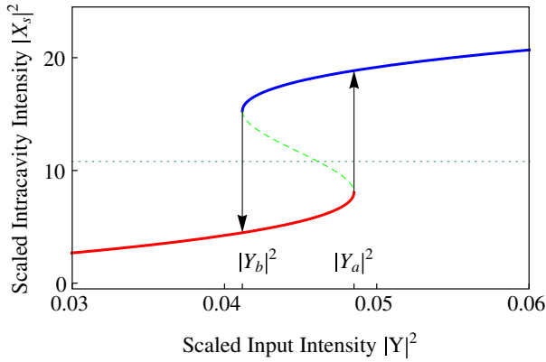
Fig. 2. Bistable dimensionless intracavity intensity |X_s|^2 as a function of the dimensionless pump intensity |Y|^2 for T = 0.01 , initial offset \delta = -0.0035 and \beta = 0.0002 . In real units, and for the parameters considered here, the threshold intensities for the bistable domain are 0.74 mW and 0.87 mW. The steady-state position of the mirror is likewise bistable.
