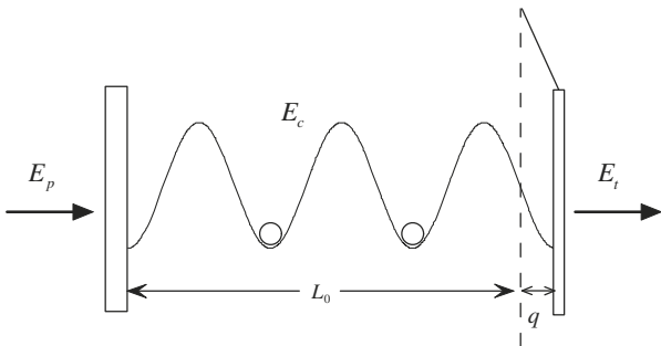
Fig. 1. A Fabry–Pérot cavity with a movable mirror displaced from its equilibrium position by q . E_p , E_c and E_t are the pump, cavity and transmitted light amplitudes, respectively.
