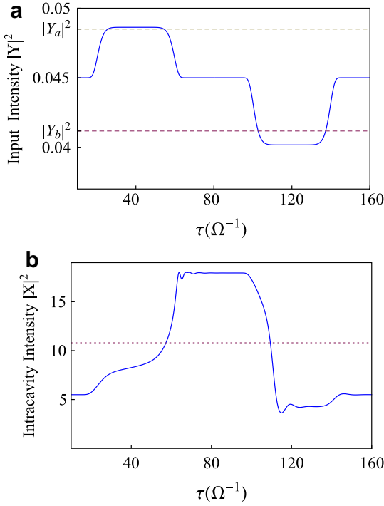
Fig. 4. (a) Input intensity |Y|^2 as a function of dimensionless time \tau . The two dashed lines label the critical intensities at the beginning and the end of the bistable region. (b) Evolution of the intracavity intensity |X|^2 controlled by |Y|^2 . Here \gamma = 0.5 and the other parameters are as in Fig. 2. The dotted line labels the critical depth of the atomic phase transition.
