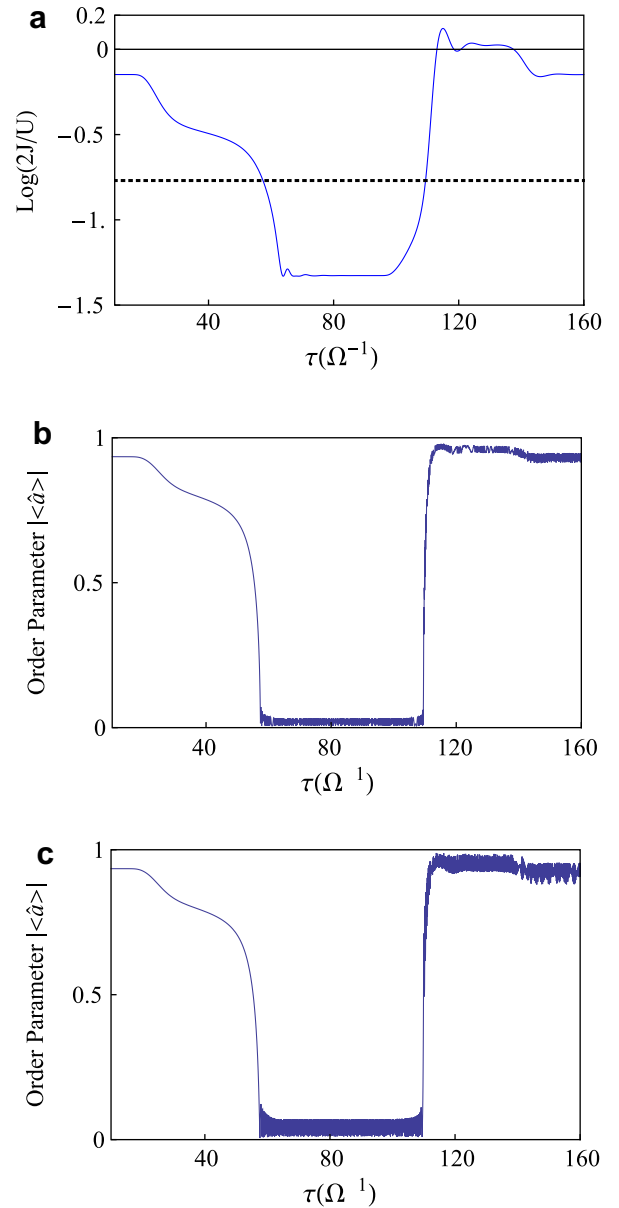
Fig. 5. (a) 2J(t)/U(t) as a function of the dimensionless time \tau . The dotted line indicates the critical value 2J/U = 0.17 , corresponding to the potential depth 10.8E_r for our parameters, for the superfluid and to Mott insulator phase transition. (b) Dynamics of the superfluid order parameter |\langle a \rangle| during the transition from the superfluid to the Mott insulator and back to the superfluid. Here \lambda_p = 985 nm and \omega_r = E_r/\hbar = 2\pi \times 8.9 kHz for ^{23}\text{Na} . The mass and vibration frequency of the mirror are M = 0.078 g and \Omega = 2\pi \times 10 Hz, respectively. In real units, the full cycle through the bistable loop takes 2.5 s. (c) Same as (b) but for M = 0.031 g and \Omega = 2\pi \times 50 Hz.
