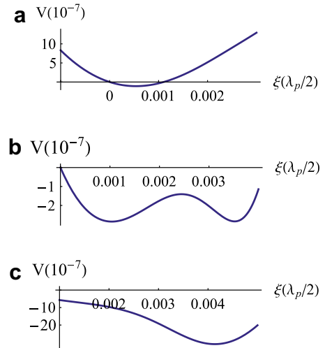
Fig. 3. Potential V(\xi) for: (a) input intensity |Y|^2 = 0.03 ; (b) |Y|^2 = 0.044 ; and (c) |Y|^2 = 0.06 . Other parameters are the same as in Fig. 2. All variables are dimensionless.
