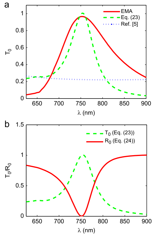
Fig. 2. Zeroth order (a) transmission, and (b) transmission and reflection spectra of a gold grating for P=75 nm, w=20 nm, h=198 nm, n_s=1 , and \theta=0^\circ .
