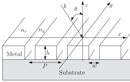
Fig. 1. 1D lamellar grating.
