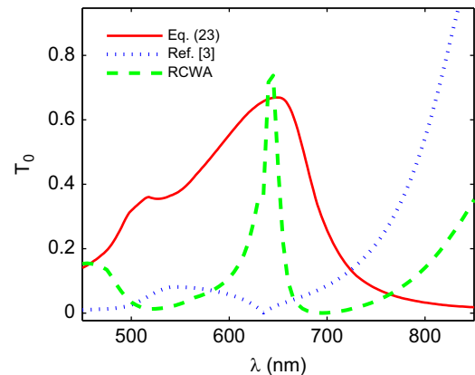
Fig. 4. Zeroth order transmission for P = 418 nm, w = 50 nm, h = 209 nm, n_s = 1.52 , \theta = 0^\circ and the ridge metal is gold.
