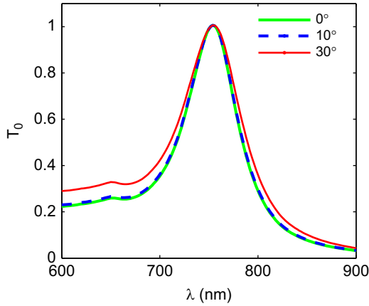
Fig. 3. Zeroth order transmission at different incidence angle for the same grating parameters of Fig. 2.
