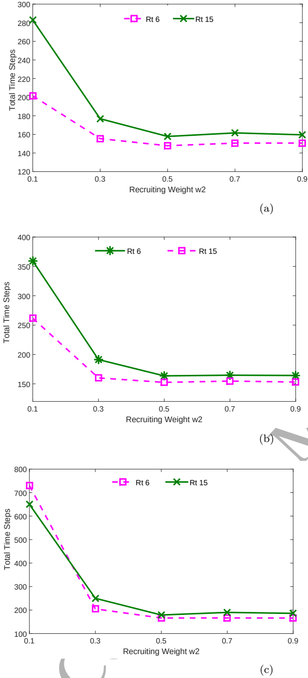
Figure 14: Evaluation of the total time steps to execute the mission in 50x50 squares and 40 robots and 3 robots to handle a target. (a) 15 targets to be handled. (b) 20 targets to be handled. (c) 35 targets to be handled.
