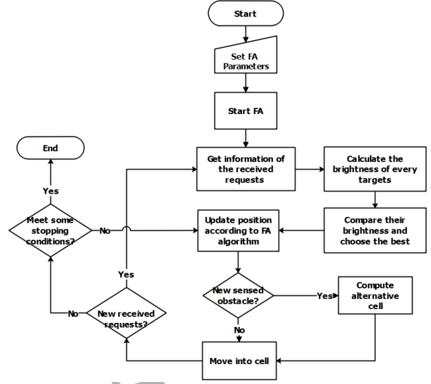
Figure 10: The flow chart of the Firefly Algorithm executed by a robot. At each step, the robots make decisions on the basis of events that can occur.
