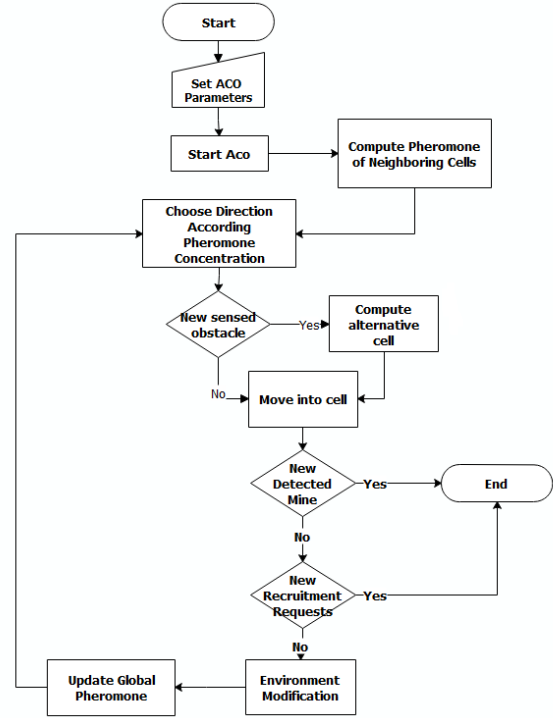
Figure 8: The flow chart of Exploration task for a robot
