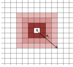
Figure 7: Example of pheromone diffusion. When a robot moves into new cell, it spreads the pheromone within a certain distance R_s . The intensity of pheromone decays according to the distance from the cell.
