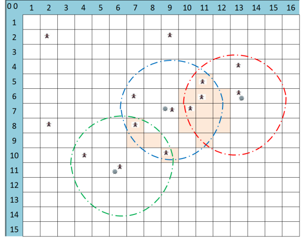
Figure 9: Example of an overlap region in which some robots are in the wireless ranges of different coordinator robots and thus they must decide towards which target to move, according to the Firefly-based strategy.
