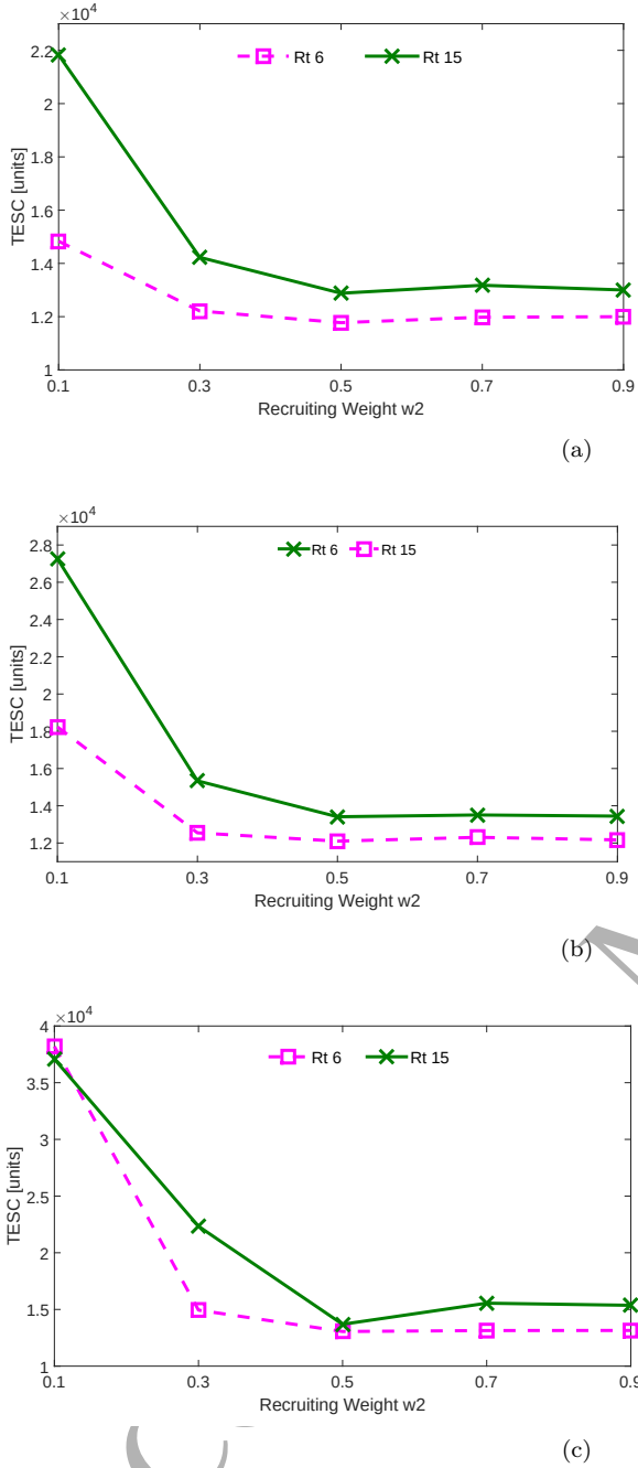
Figure 15: Evaluation of the total energy consumed by the system in 50x50 squares and 40 robots and 3 robots to treat a target. (a) 15 targets (b) 20 targets (c) 35 targets .
