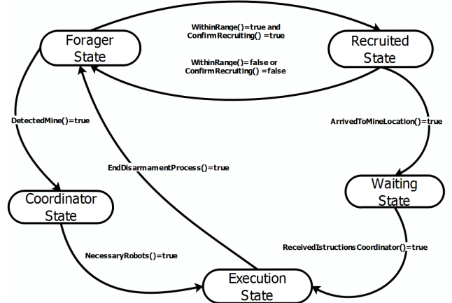
Figure 6: State transition logic for robots at each time step. WithinRange() is a function returning True when the robot is within the communication range of a coordinator robot. Confirm Recruiting() is a function returning True if the robot decides to get involved in the disarmament process of a target. ArrivedToMineLocation() and ReceivedInstructionsCoordinator() are two functions returning True if the robot is arrived to a target's location and received the command to start the disarmament process by the coordinator, respectively. NecessaryRobot() returns True if all needed robots ( R_{min} ) have arrived at the target's location.
