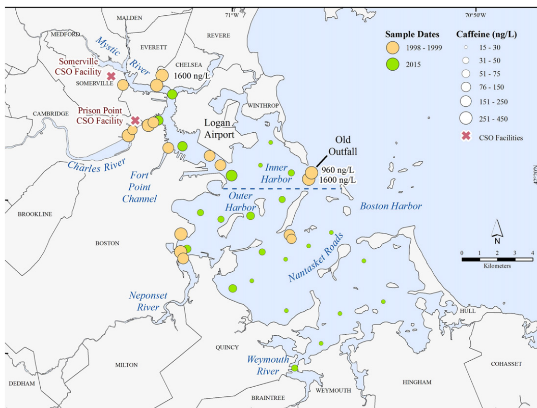
Fig. 1. Caffeine concentrations in Boston Harbor. Size of marker denotes concentration.
