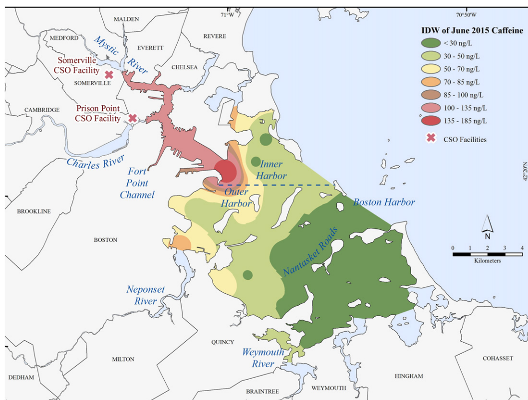
Fig. 2. Inverse distance weighting spatial analysis of 2015 caffeine data.
