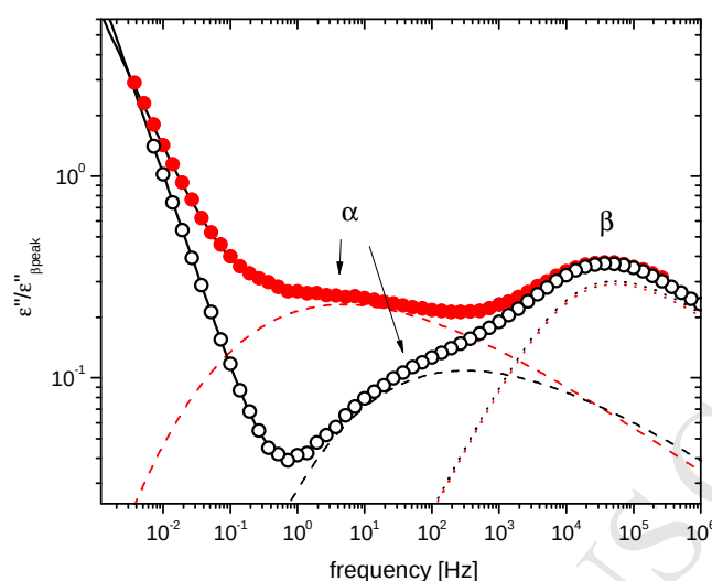
Figure 1. Dielectric loss spectra for bulk PMMA (solid circles; T = 406.6 K) and multilayered PMMA with 8 nm layer thickness (open circles; T = 406.8 K). For the multilayer sample, the permittivity of the PMMA was extracted from the measured permittivity by correcting for the PC contribution as discussed in the text. There is a significant slowing down of the \alpha process under confinement, whereas the \beta peak frequency is unaffected. The ordinate values were normalized by the maximum of the \beta peak. The rise of the dielectric loss at low frequency reflects conduction loss from ionic impurities. The dashed and dotted lines are the respective contributions of the \alpha and \beta process as obtained from the fit.
