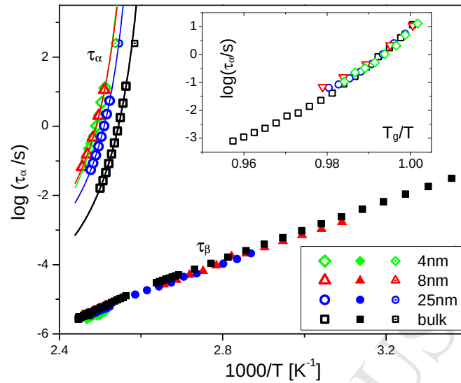
Figure 2. Arrhenius plot of the dielectric relaxation times for bulk PMMA (squares) and three PMMA multilayers (diamonds – 4 nm layer thickness; triangles – 8 nm; circles – 25 nm). Open symbols are for the \alpha relaxation and filled symbols for the \beta relaxation. The \alpha relaxation time from MDSC for each multilayer sample is also shown (dotted symbols at \log \tau_\alpha = 2.40 ). In the inset are \tau_\alpha versus inverse T_g -normalized temperature, using \tau_\alpha(T_g) = 10 s, showing that the fragilities of the four samples are essentially the same.
