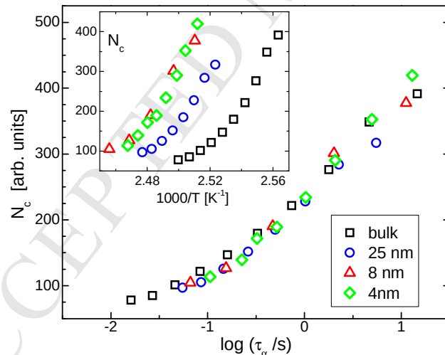
Figure 3. Number of dynamically correlated units versus the \alpha relaxation time for bulk and nanoconfined PMMA samples. Notwithstanding the large changes of N_c due to confinement (inset), the dependence of N_c on \tau_\alpha is the same as for the bulk PMMA. Error bars are smaller than the symbol size.
