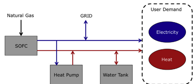
Fig. 1. General scheme of the system proposed here with the main component and energy flows: fuel (black), electricity (blue) and heat (red). (For interpretation of the references to color in this figure legend, the reader is referred to the web version of this article.)
