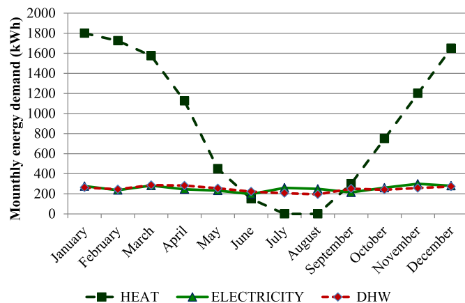
Fig. 3. Average monthly demand on electricity, heat and domestic hot water (DHW) for a resort located in Denmark.
