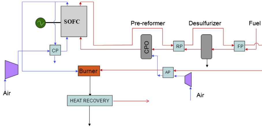
Fig. 2. Representation of the SOFC system. CP = cathode preheater, FP = fuel preheater, AP = air preheater, RP = reformer preheater.
