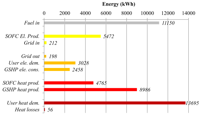
Fig. 8. Energy flux for the ELF 2-kW operation strategy.
