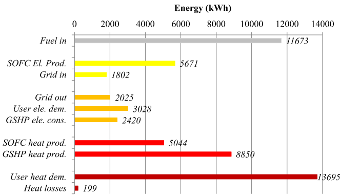
Fig. 10. Energy flux for the ELF CO strategy.
