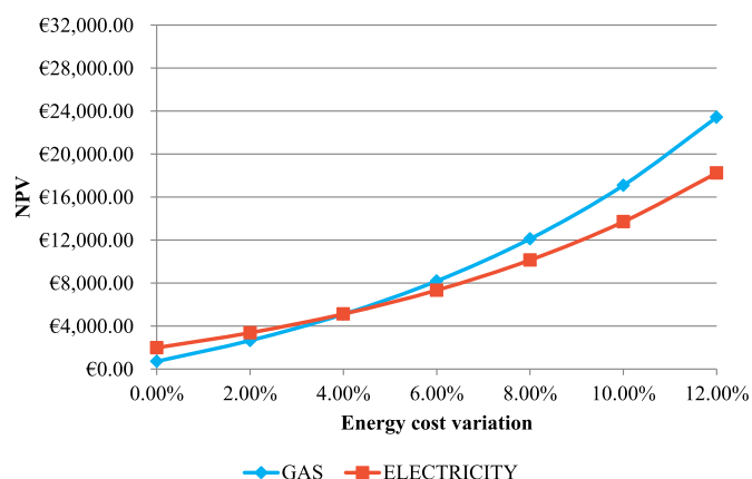
Fig. 16. Sensitivity analysis on the energy cost with ELF 1 kW.
