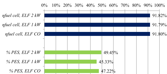
Fig. 7. Fuel cell efficiency and %PES for all of the strategies.
