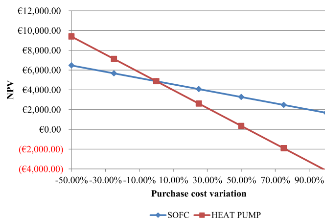
Fig. 15. Sensitivity analysis on the purchase cost with ELF 1 kW.
