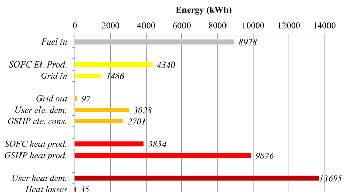
Fig. 9. Energy flux for the ELF 1-kW operation strategy.
