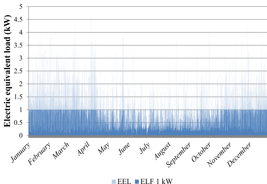
Fig. 5. Electric equivalent load with ELF 1 kW, annual overview. ELF 1 kW follows EEL until it is lower or equal to 1 kW (the darker color). (For interpretation of the references to color in this figure legend, the reader is referred to the web version of this article.)
