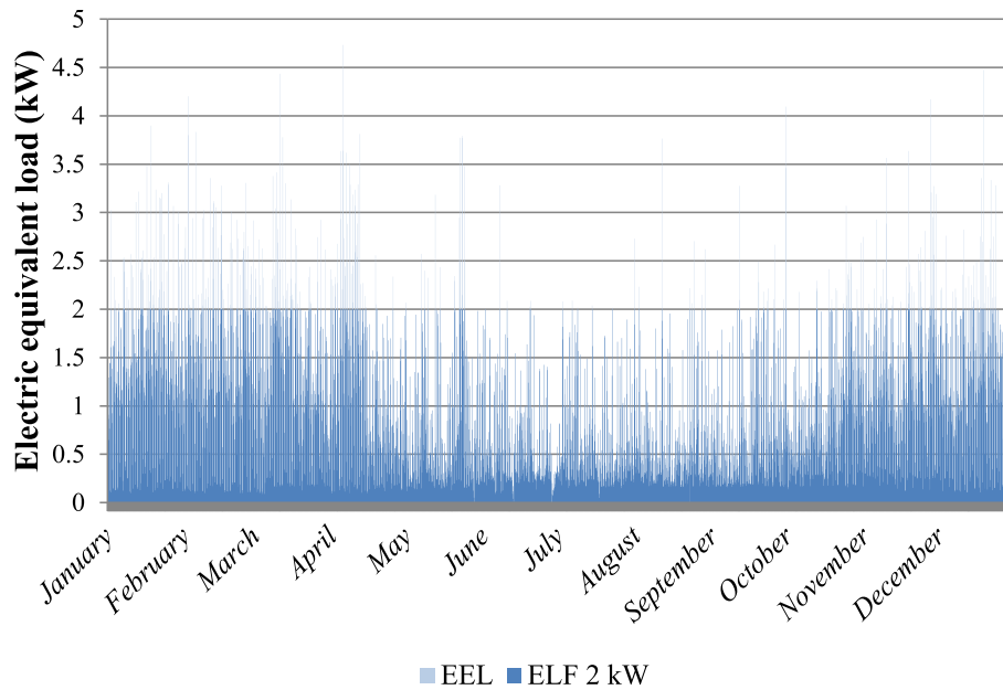
Fig. 4. Electric equivalent load with ELF 2 kW, annual overview. ELF 2 kW follows EEL until it is lower or equal to 2 kW (the darker color). (For interpretation of the references to color in this figure legend, the reader is referred to the web version of this article.)
