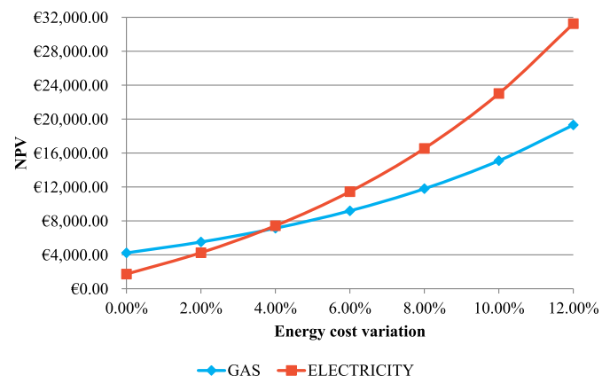
Fig. 13. Sensitivity analysis on the energy cost with ELF 2 kW.
