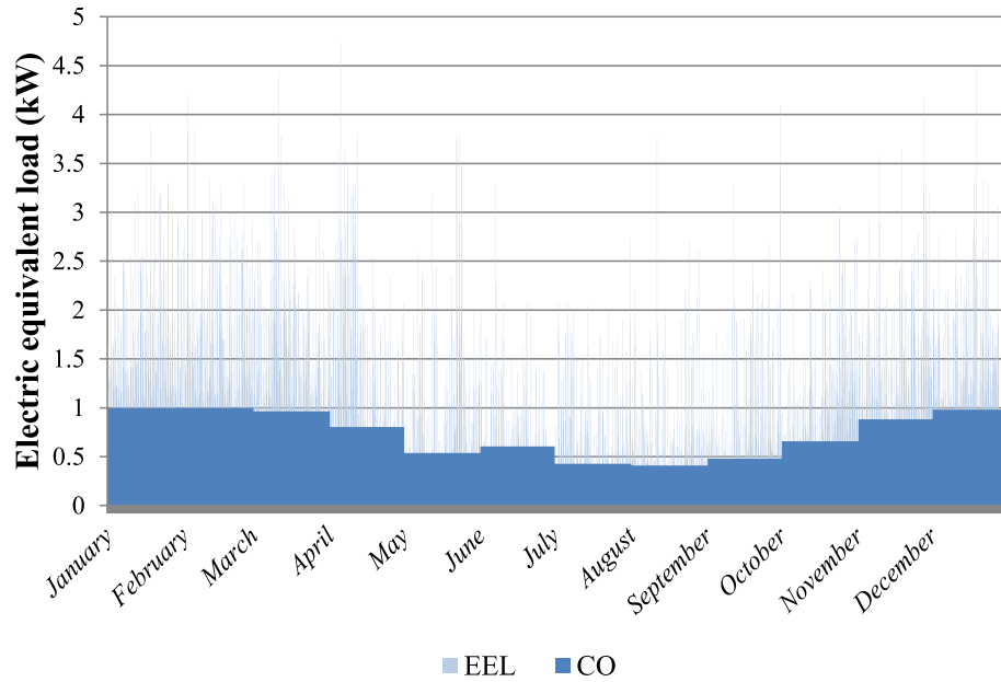
Fig. 6. Electric equivalent load with continuous operation (CO) strategy, annual overview. CO follows a monthly average of EEL (the darker color). (For interpretation of the references to color in this figure legend, the reader is referred to the web version of this article.)
