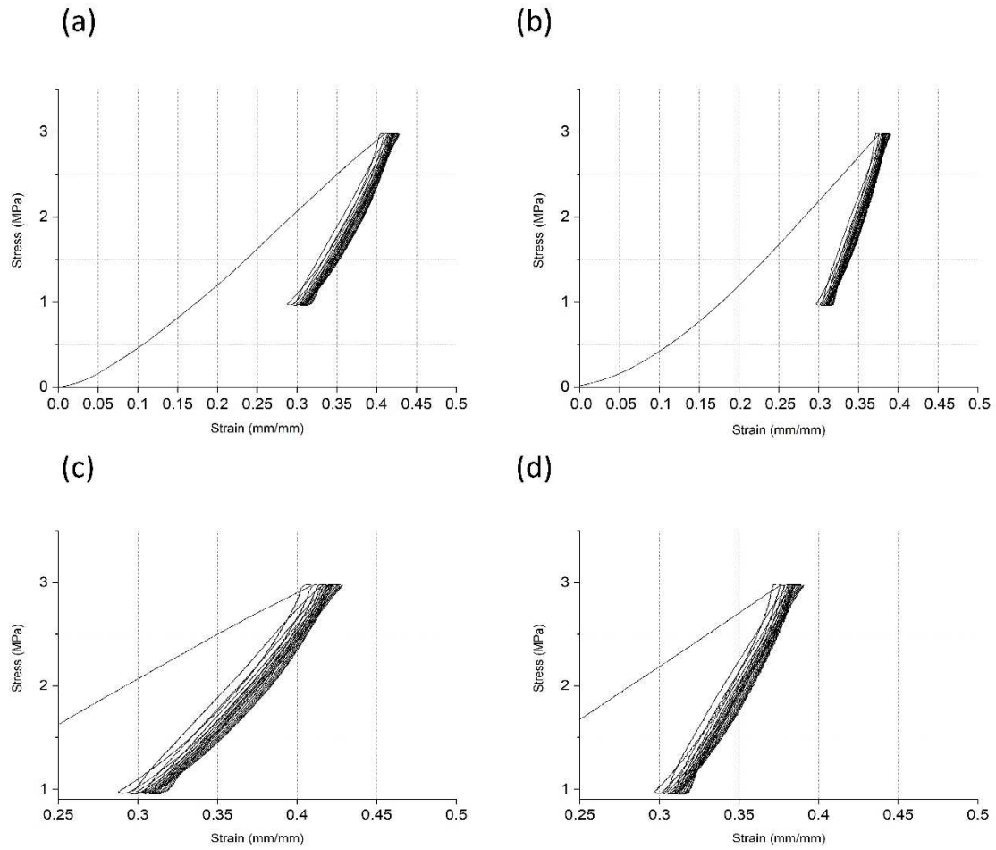
Fig. 4 The stress-strain curves of the tested (a) Toray-H-90 and (b) SGL-34-BC GDL materials. (c) and (d) are zoomed-in graphs of the cyclic compression part of the stress-strain curves for Toray-H-90 and SGL-34-BC, respectively.
