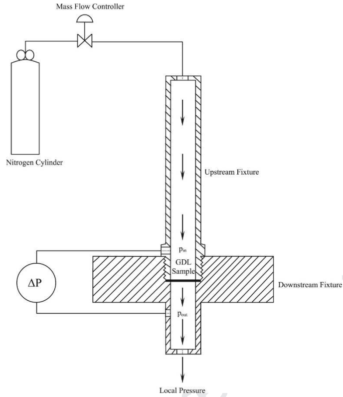
Fig. 2 A schematic of the experimental setup of the through-plane permeability. Reprinted from Ref. [32] with the permission of Elsevier.
