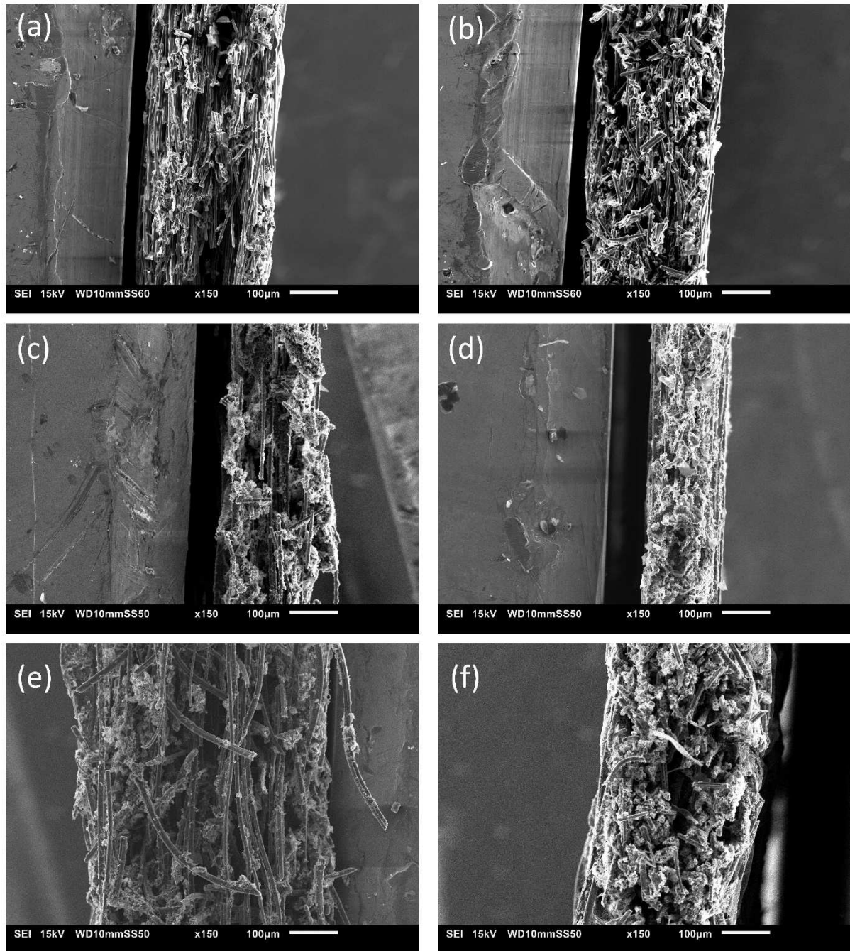
289 Fig. 6 Cross-sectional SEM images at a magnification of 150x for uncoated GDL samples before and after 290 compression, (a) uncompressed Toray-H-90 (b) Compressed Toray-H-90 (c) Uncompressed SGL-24-BA (d) 291 Compressed SGL-24-BA (e) Uncompressed SGL-10-BA (f) Compressed SGL-10-BA.
