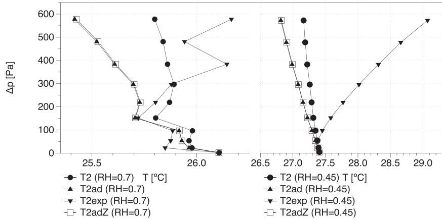
Fig. 12. Pressure drop for stationary flow for high (left) and low (right) air moisture conditions.
