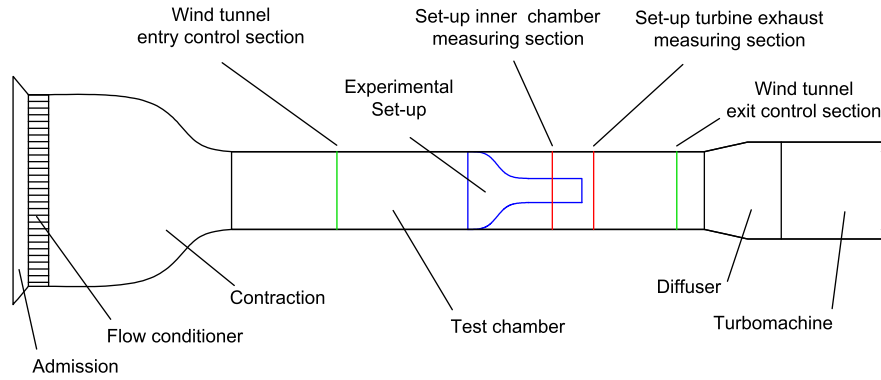
Fig. 9. Schematic reference of gauges placement.
