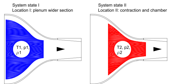
Fig. 1. Control Volume deformation of the thermodynamic system flowing through the set up. System state I & location I (left). System state II & location II (right).
