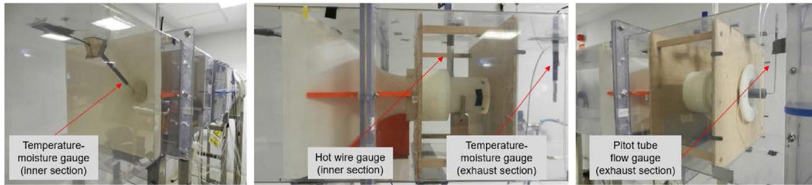
Fig. 10. Detailed view of temperature–moisture, hot wire and pitot tube flow gauges.
