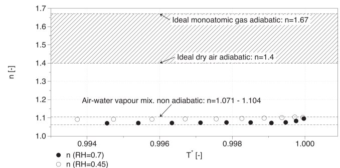
Fig. 13. Polytopic exponent n for the compression process vs. non dimensional temperature T^* = T_2/T_1 .
