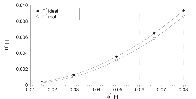
Fig. 15. Non dimensional flow vs. non dimensional power output in Pico Plant case study for both the real gas model and the classical theory in several sea states.
