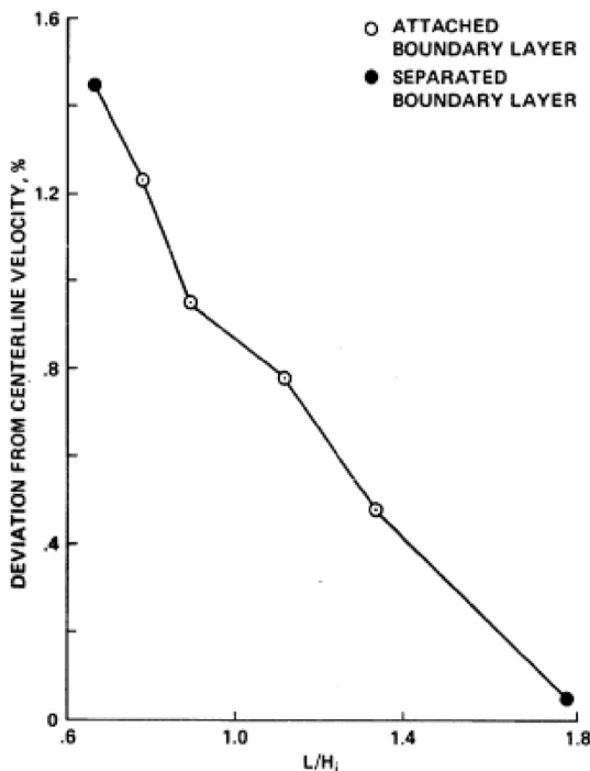
Fig. 5. Velocity deviation from centerline values vs. L/H_i , 61.
