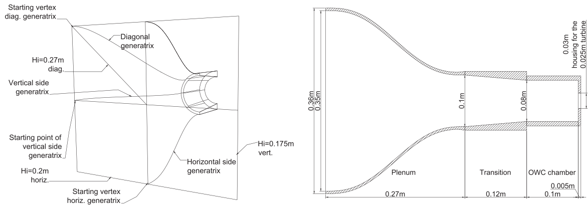
Fig. 6. Plenum generatrix scheme (left) and set-up longitudinal section (right).
