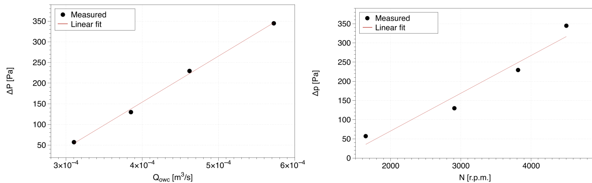
Fig. 8. Pressure drop vs. air flow for the experimental set up (left) and pressure drop vs. turbine speed for the experimental set up (right).
