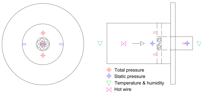
Fig. 11. Pressure taps, temperature–humidity gauges and hot wire in the experimental set-up.
