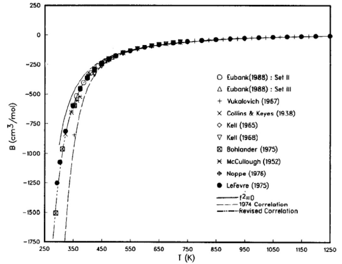
Fig. 3. Second virial coefficient, B , 60. The ordinary range of temperature for an OWC system falls under 350 K, corresponding to the leftmost region of the temperature axis.
