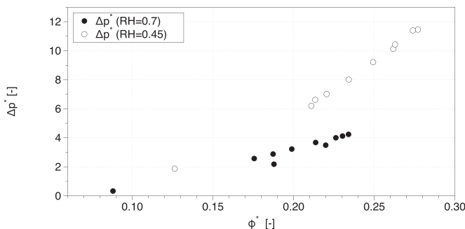
Fig. 14. Non dimensional flow vs. pressure drop for both high and low moisture conditions.
