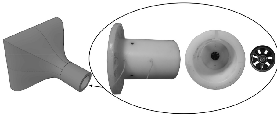
Fig. 7. OWC turbine, OWC chamber and its relative position with respect to the plenum.
