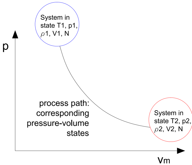
Fig. 2. System process in the p - V thermodynamic space.
