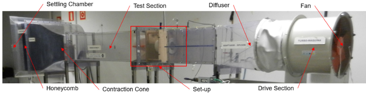
Fig. 4. Wind tunnel set up.
