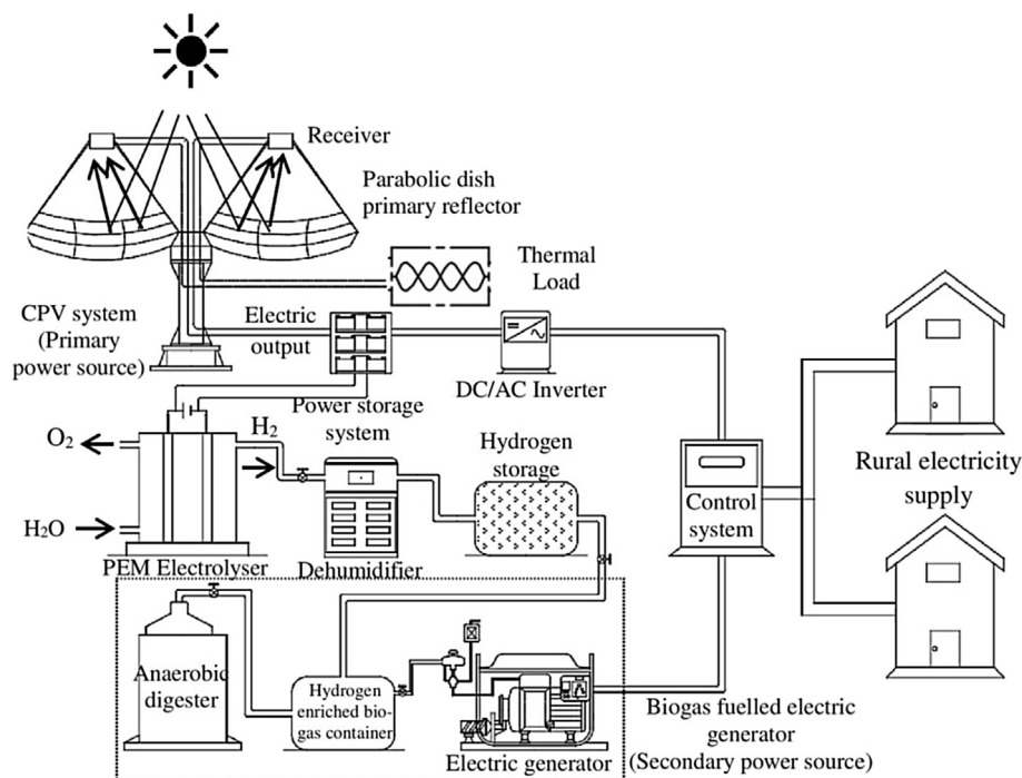
Fig. 1. The conceptual layout of Bio-CPV.
