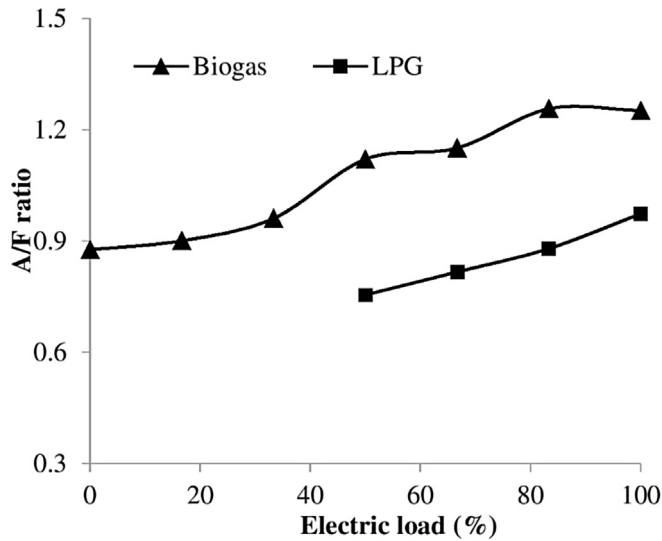
Fig. 16. Effect of loading on relative Air/Fuel Ratio.
