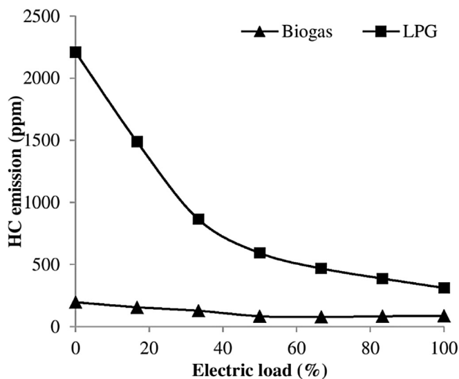
Fig. 13. Effect of loading on hydrocarbon (HC) emission.
