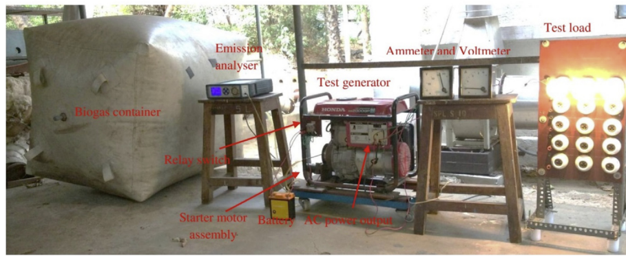
Fig. 3. Experimental set up of LPG generator functioning using biogas.
