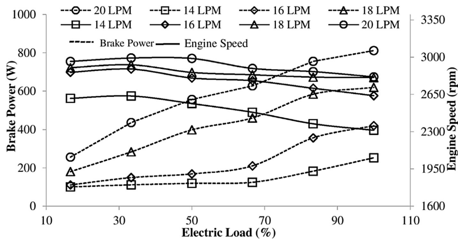
Fig. 4. Variation of brake power and engine speed with electric load.
