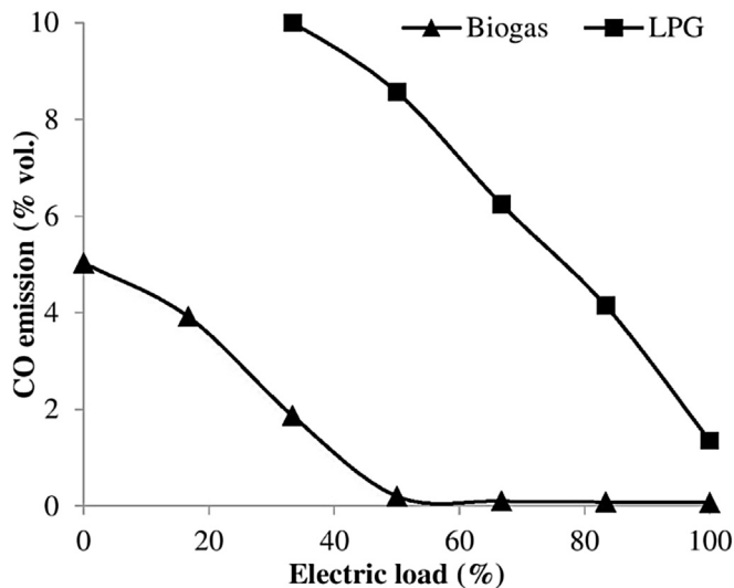
Fig. 12. Effect of loading on carbon monoxide (CO) emission.
