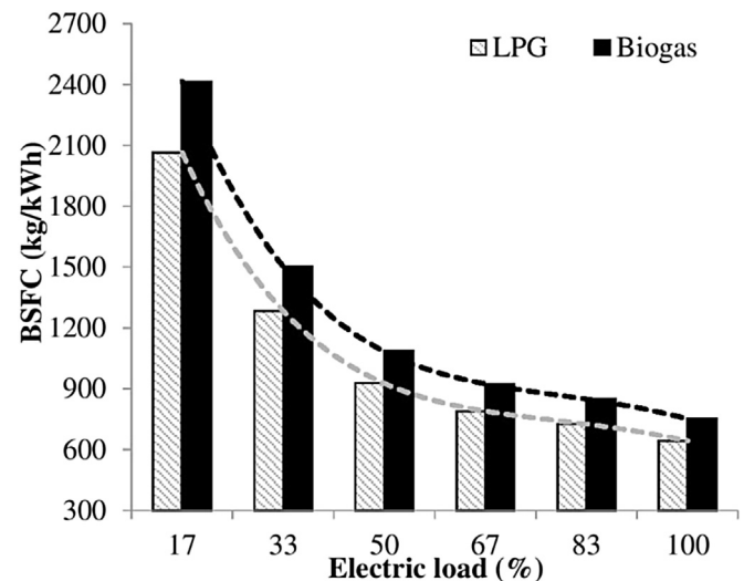
Fig. 10. Comparative variation of brake specific fuel consumption with electric load.
