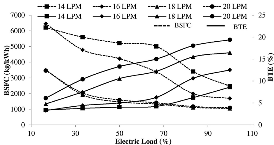
Fig. 5. Variation of brake specific fuel consumption and brake thermal efficiency with electric load.
