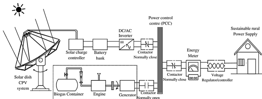
Fig. 17. Concept of integrating biomass- CPV hybrid renewable energy system.
