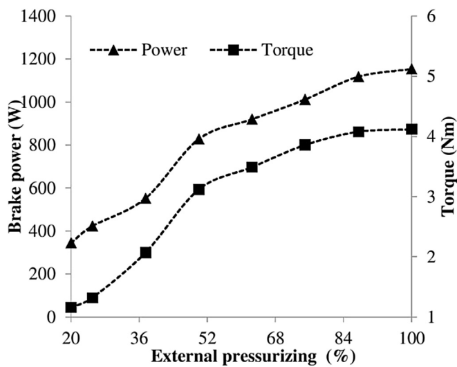
Fig. 6. Effect of external pressurizing on Brake power and torque.
