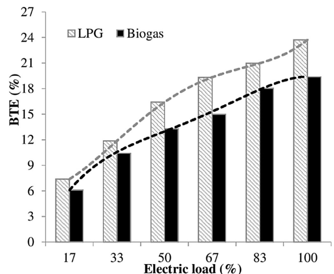
Fig. 11. Comparative variation of brake thermal efficiency with electric load.
