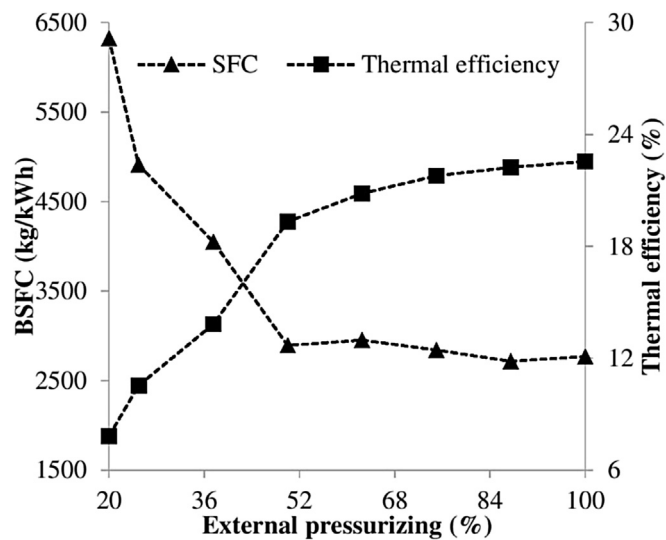
Fig. 7. Effect of external pressurizing on BSFC and BTE.
