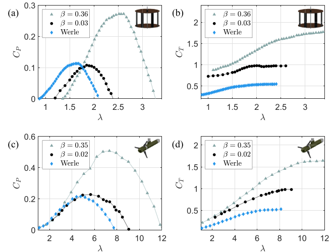
Fig. 7. The results of applying Werle's correction to the confined performance data from the cross-flow (a, b) and axial-flow (c, d) turbines.
