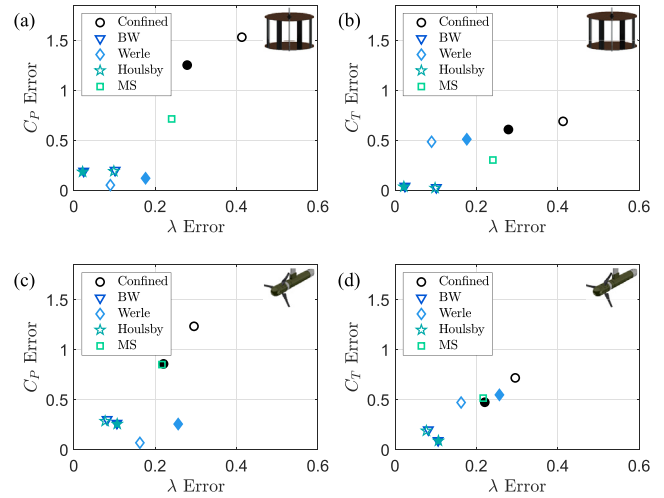
Fig. 10. Blockage correction error for the cross-flow (a, b) and axial-flow (c, d) turbines, relative to unconfined data. Filled markers indicate error averaged over full curves, while open markers indicate error at peak C_p .
