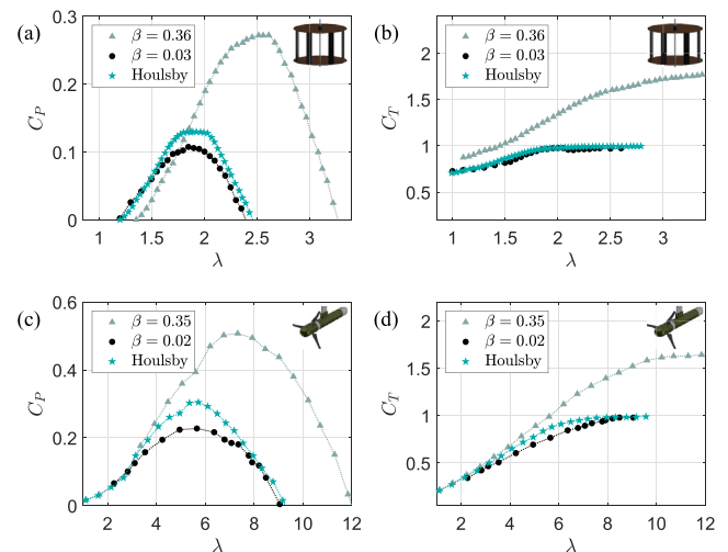
Fig. 8. Housby et al.'s method applied to the confined performance data from the cross-flow (a, b) and axial-flow (c, d) turbines.
