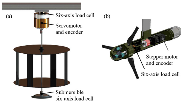
Fig. 1. Renderings of the cross-flow (a) and axial-flow (b) experimental turbines used in this study.
