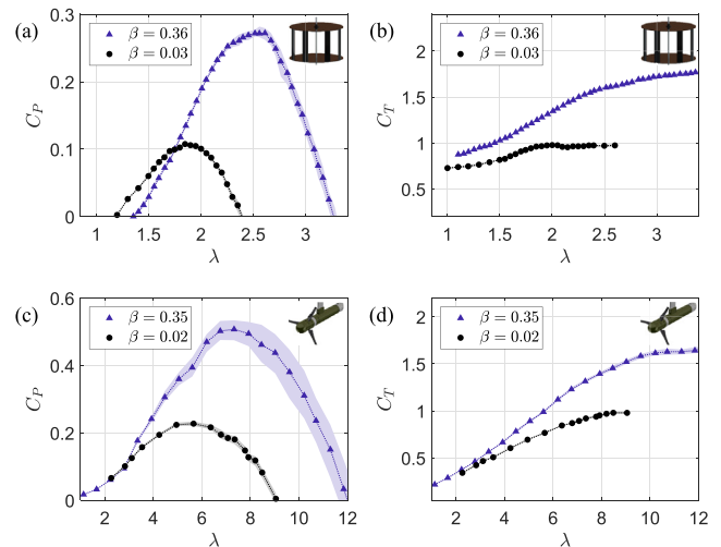
Fig. 5. Confined and unconfined power and thrust coefficients for the cross-flow (a, b) and axial-flow (c, d) turbines. The shading represents the measurement uncertainty at each tip-speed ratio, as estimated from the interquartile range of cycle-average performance. In some instances, the uncertainty range is smaller than the plot markers, and therefore not visible.
