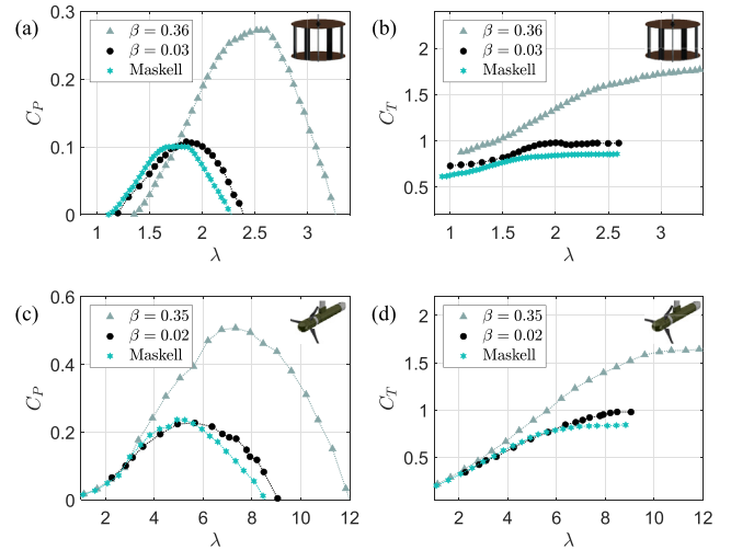
Fig. 12. Application of a blockage correction inspired by the bluff body theory of Maskell to the confined performance data from the cross-flow (a, b) and axial-flow (c, d) turbines.
