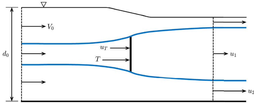
Fig. 4. Streamtube model of an actuator disk in open channel flow with a deformable free surface.
