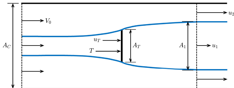
Fig. 3. Streamtube model of an actuator disk in closed channel flow with no free surface.
