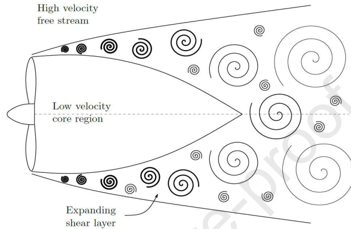
Figure 1: A schematic of the wake description. Flow direction is from left to right.
