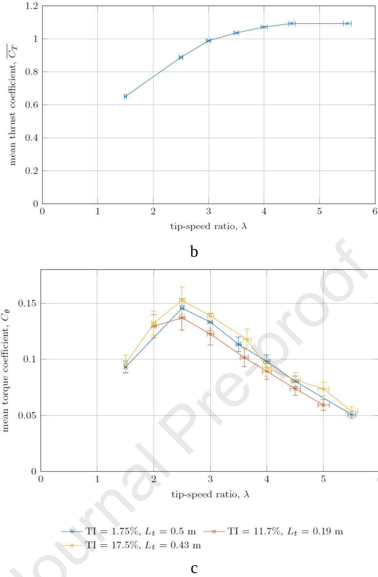
Figure 7 Flume results for a) C_P vs. \lambda . b) C_T vs. \lambda . c) C_\theta vs. \lambda
