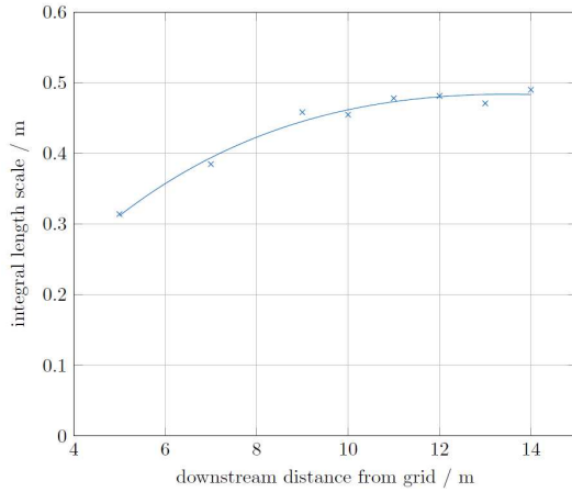
355 Figure 6: Flow characteristics downstream of the fine and coarse grids, measured at the centre 356 of the cross-sectional area of the flume.
