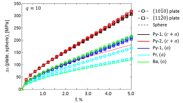
Fig. 5. CRSS increment of slip systems due to Orowan strengthening by \{10\bar{1}0\} and \{11\bar{2}0\} plate and spherical precipitates, as observed in Mg alloy, WE43-T5 [19]. The three precipitate morphologies are represented by marker shapes circle, square and no marker respectively. The five slip systems are represented by different colors of markers and dashed lines. Plate size is D=20 nm and T=2 nm, spheres have the same volume as plate precipitates.
