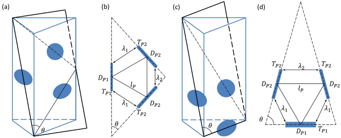
Fig. 1. Precipitate plates on \{10\bar{1}0\} planes are intersected by slip plane (a) (11\bar{2}2) and (c) (10\bar{1}1) respectively. (b) Projection of the intersected precipitates on the (11\bar{2}2) plane. (d) Projection of the intersected precipitates on the (10\bar{1}1) plane. The precipitates are assumed to distribute in an equilateral triangular array on the slip plane.
