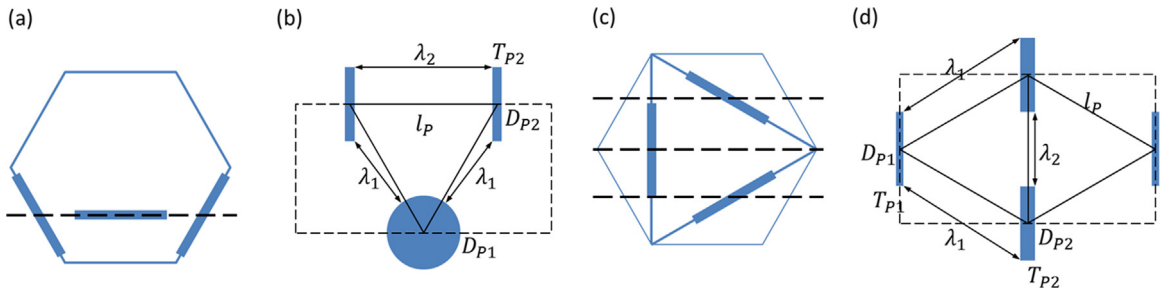
Fig. 2. Precipitate plates on (a) \{10\bar{1}0\} planes and (c) \{11\bar{2}0\} planes are intersected by slip plane (10\bar{1}0) viewing perpendicular to the (0001) basal plane. (b) Projection of the intersected \{10\bar{1}0\} precipitates on the slip plane. (d) Projection of the intersected \{11\bar{2}0\} precipitates on the slip plane. The precipitates are assumed to distribute in an equilateral triangular array on the slip plane.
