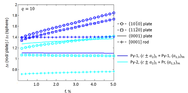
Fig. 6. Variation of the normalized CRSS increment with the volume fraction of four precipitates, whose aspect ratio q is 10. The slip systems considered inside twin comprise the transmuted \langle c\pm a_2 \rangle dislocations on first order (Py-1) and second order (Py-2) pyramidal planes.
