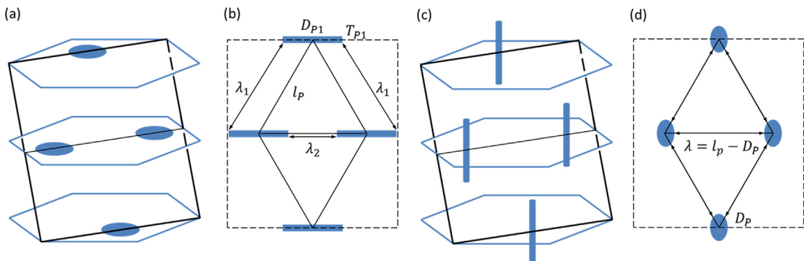
Fig. 3. (a) Precipitate plates on \{0001\} planes and (c) [0001] rods are intersected by slip plane \{11\bar{2}2\} . (b) and (d) are projections of the intersected precipitates on the slip plane. The precipitates are assumed to distribute in an equilateral triangular array on the slip plane.
