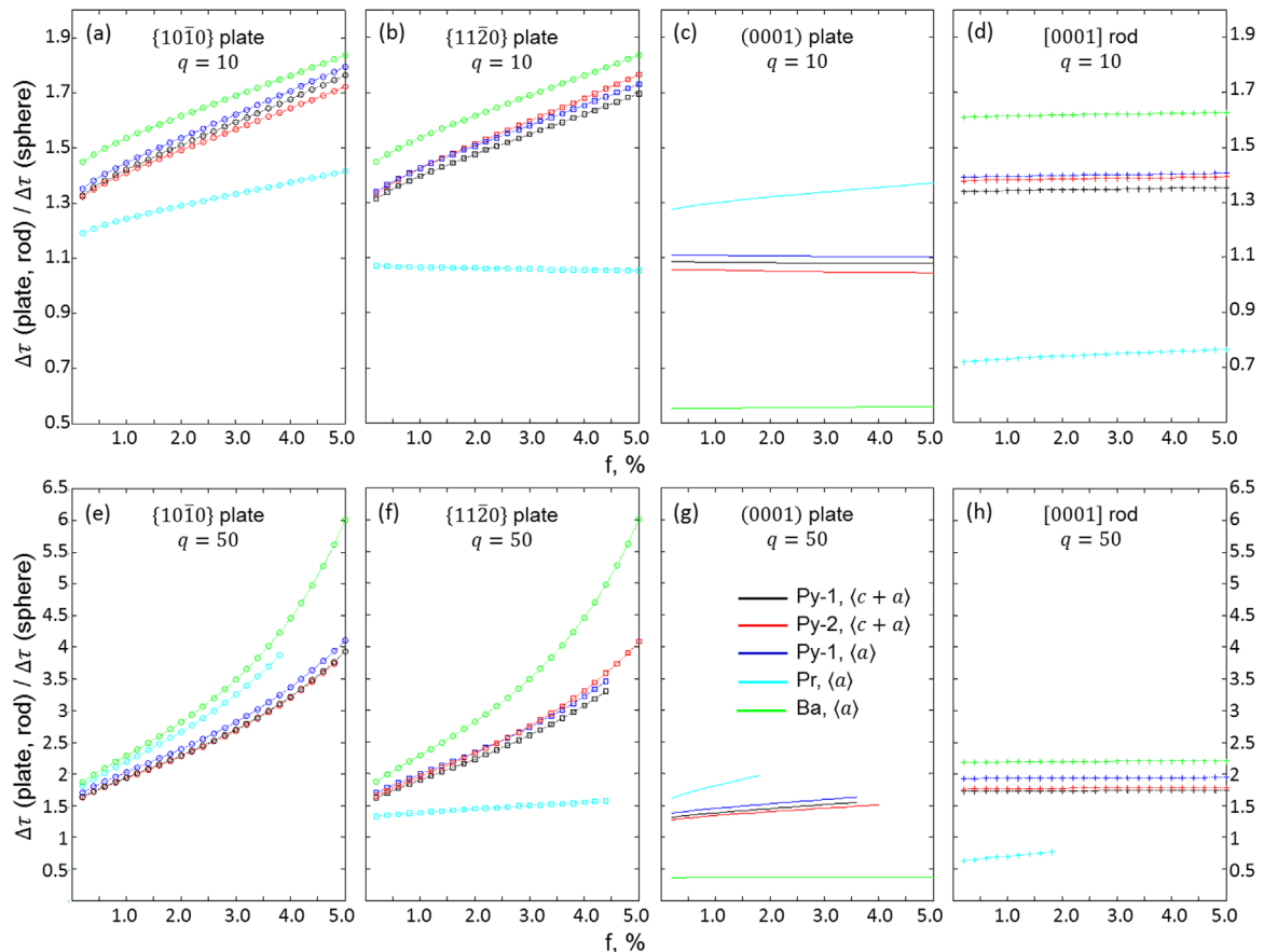
Fig. 4. Variation of the normalized \Delta\tau with volume fraction for five slip systems strengthened by (a) and (e) \{10\bar{1}0\} plate, (b) and (f) \{11\bar{2}0\} plate, (c) and (g) (0001) plate, (d) and (h) [0001] rod. The slip systems are represented by curves in different colors as indicated in (g). Two aspect ratios of precipitates are used q = 10 (a–d) and q = 50 (e–h).
