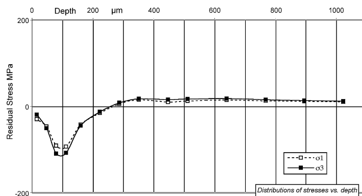
Fig. 5. Principal stresses determined using hole drilling for the as-peened sample.
