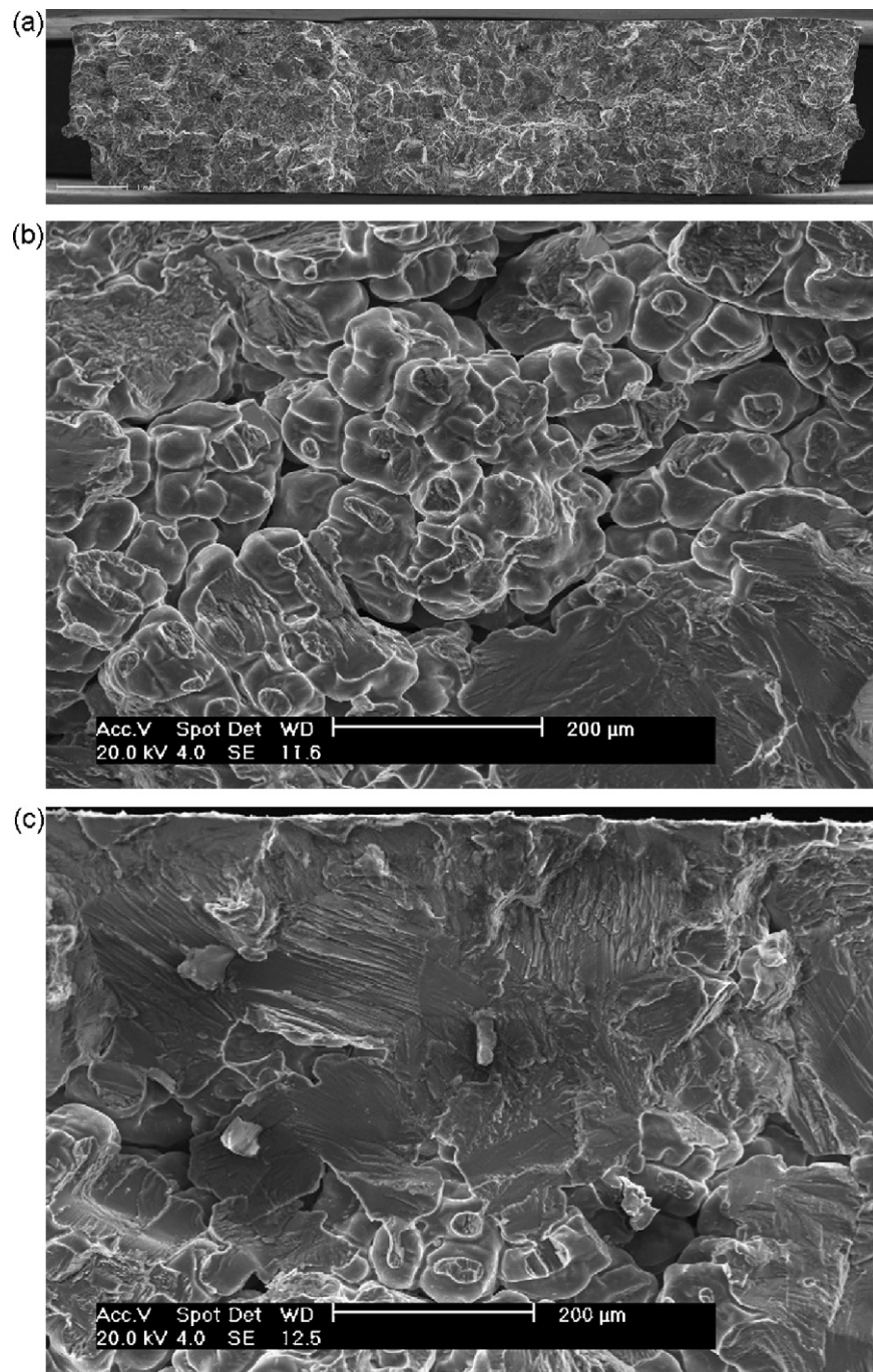
Fig. 8. (a) Fracture surface of a shot-peened sample. (b) Shrinkage porosity on the fracture surface of (a). (c) Crystallographic slip near the fatigue initiation surface of (a).
