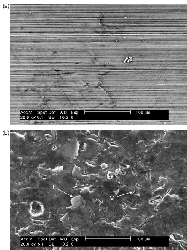
Fig. 7. (a) As-machined surface finish. (b) As-peened surface finish. Microscopic cracking (labelled M) and flaking (labelled F) are evident on the surface (arrowed).
