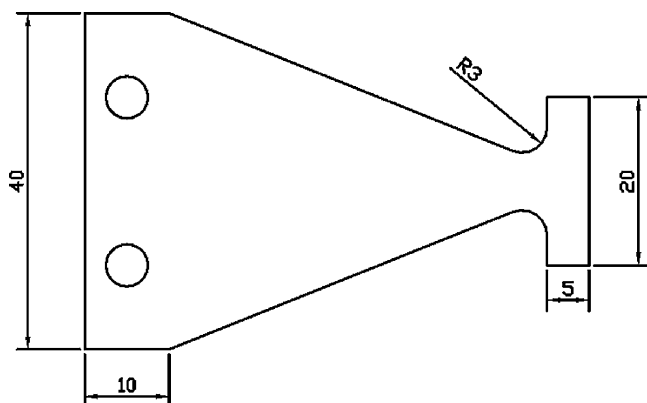
Fig. 1. Constant stress beam geometry used for the specimens. All dimensions are in mm. The holes are 5 mm diameter and the plate thickness was 3 mm.
