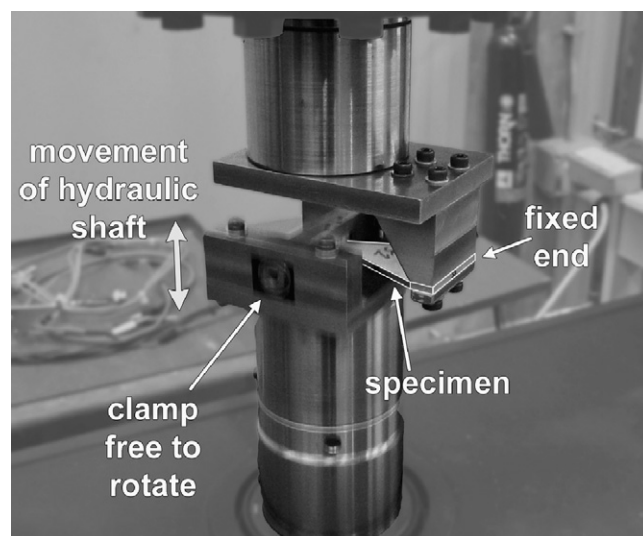
Fig. 2. Specimen positioning in the MTS servohydraulic testing machine.
