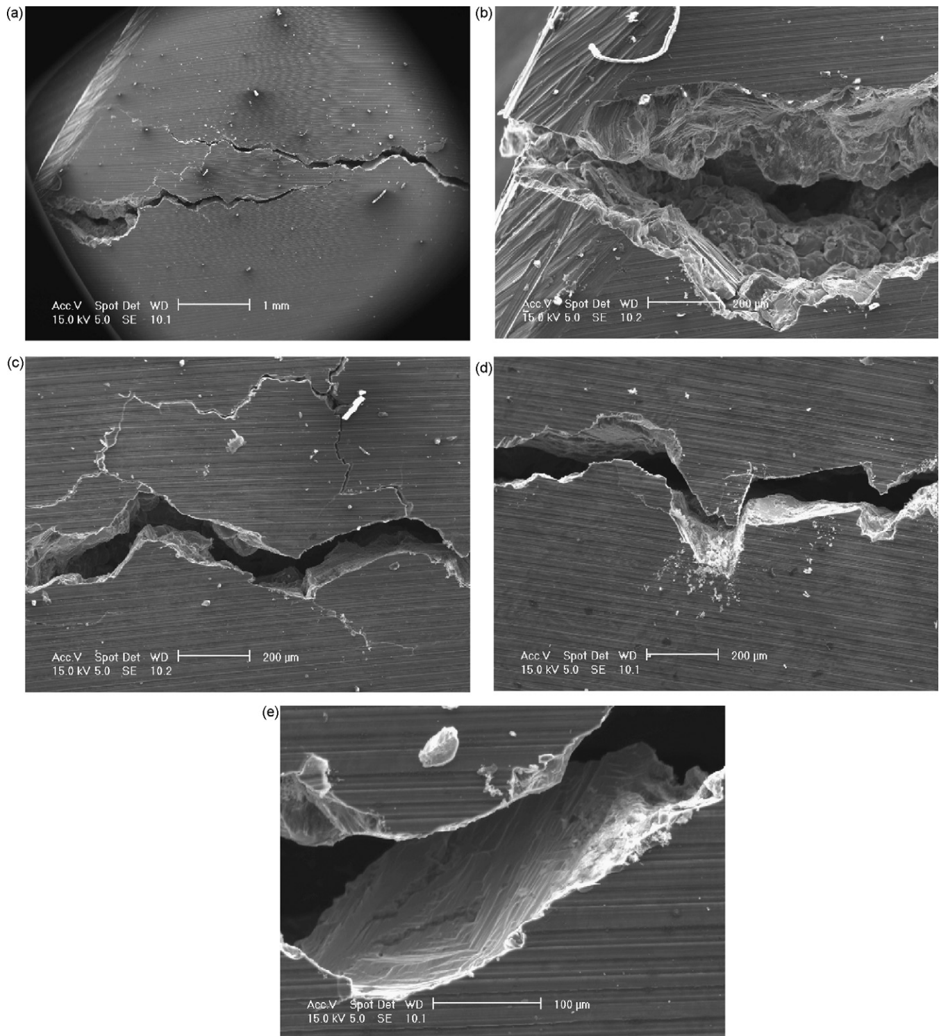
Fig. 9. (a) Low magnification image of the crack path in as-machined sample. (b) Crack initiation in a porous region of the sample. (c) Bifurcation of crack showing intergranular nature of cracking. (d) Evidence of crack following grain boundaries around the hexagonal grains. (e) Evidence of intragranular cracking as the crack follows the material's slip planes. Note also the lack of influence of the machining marks on crack propagation.
