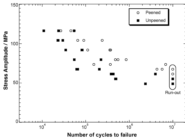
Fig. 3. Stress amplitude versus number of cycles to failure for the peened and as-machined samples ( 10^7 cycles indicates run-out).
