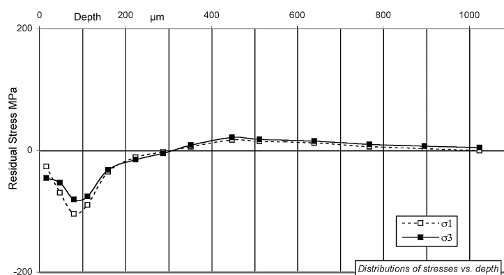
Fig. 6. Principal stresses determined using hole drilling for the peened-and-fatigued sample.
