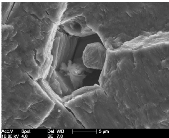
Fig. 12. Porosity formed around an inclusion during the casting process in one of the samples that was subsequently shot-peened. Note that this is a much smaller structural flaw than the region of shrinkage porosity in Fig. 8.
