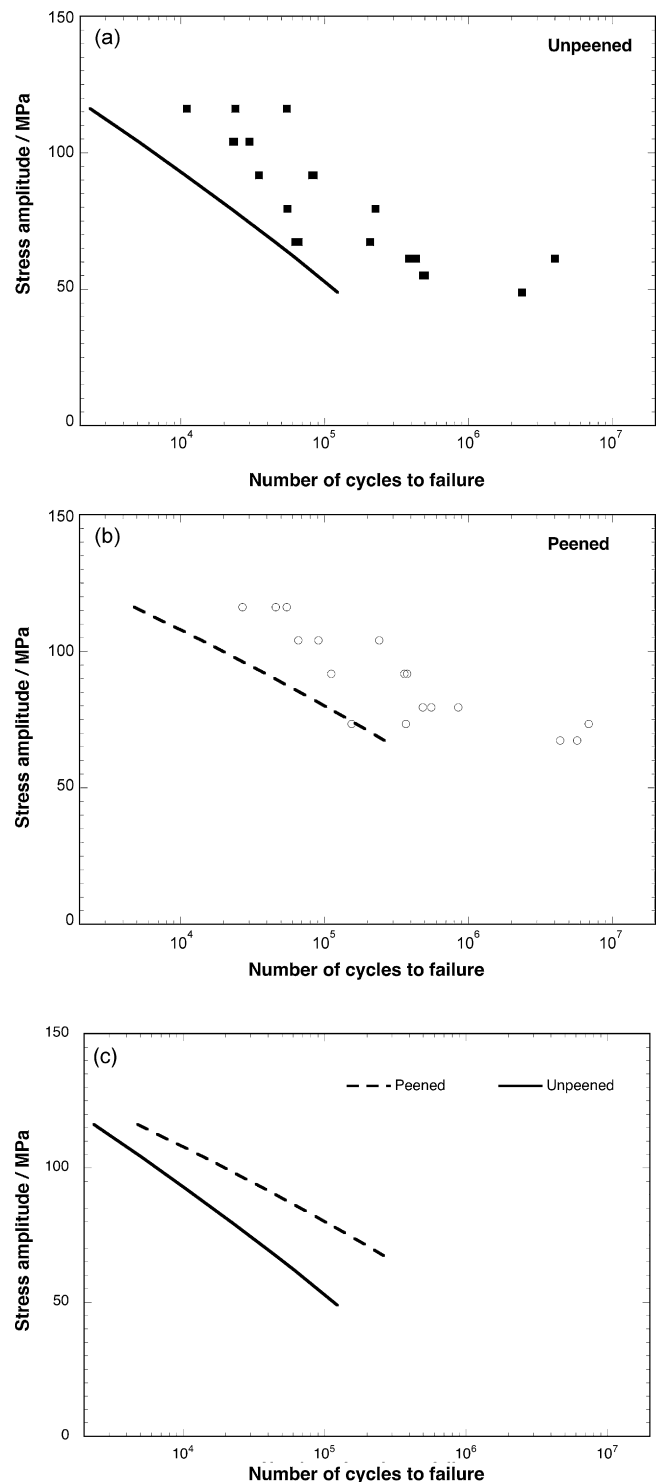
Fig. 4. (a) S-N data for the unpeened sample. The line shows the predicted S-N behaviour for a 10% failure probability, according to BS ISO 12107. The run-out samples were not used in the calculation. (b) S-N data for the peened sample. The line shows the predicted S-N behaviour for a 10% failure probability, according to BS ISO 12107. The run-out samples were not used in the calculation. (c) Comparison of the 10% failure probability predictions for the unpeened and peened specimen data.
