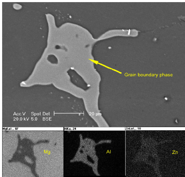
Fig. 10. Backscattered electron image of the grain boundary phase observed in a polished A8 specimen and corresponding energy dispersive X-ray maps for magnesium, aluminium and zinc. It can be seen that the aluminium and zinc alloying additions have segregated to the grain boundaries.
