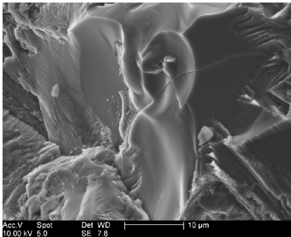
Fig. 11. Crack running through the grain boundary phase on the fracture surface of one of the shot-peened specimens.
