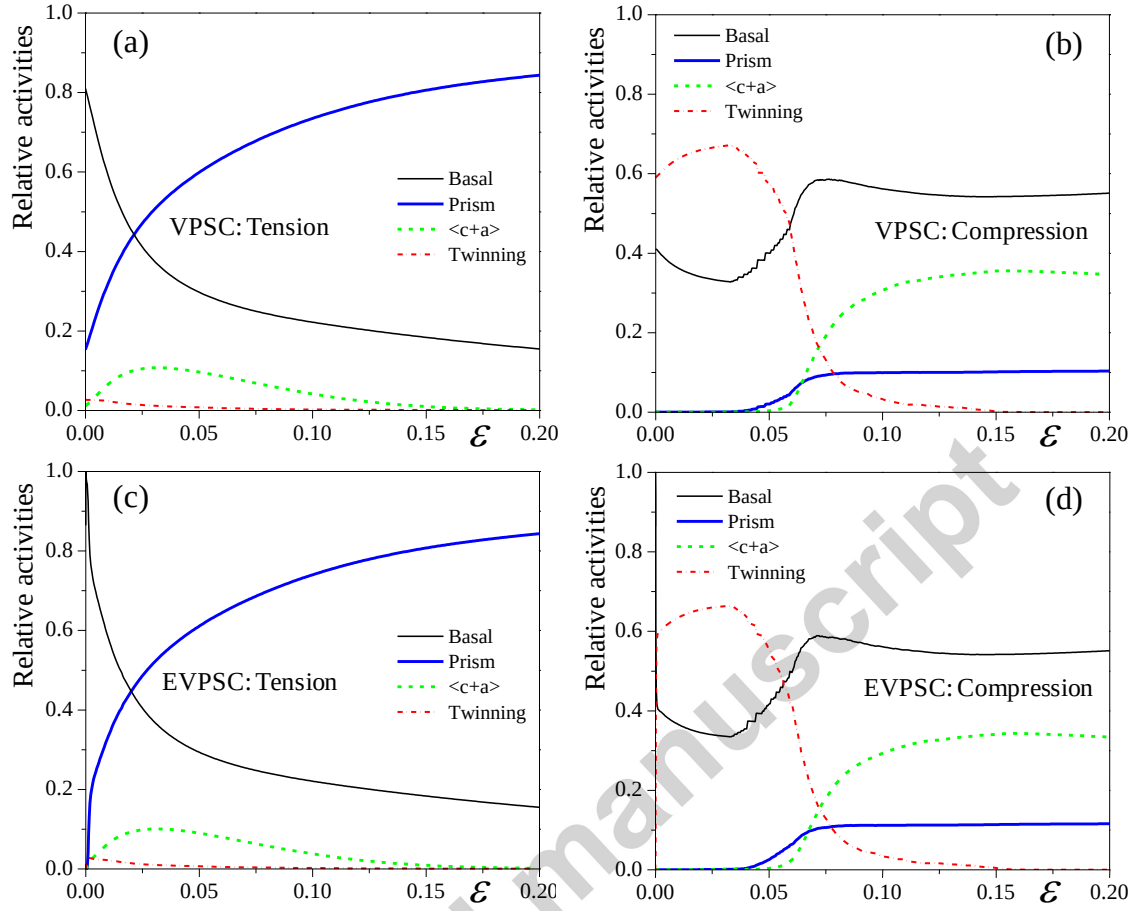
Figure 15. Deformation mechanism activity plots for tension (a & c) and compression (b & d) strained along ED for the VPSC and EVPSC calculations, respectively. Each self-consistent scheme employs the TDT twinning model and the N_{eff} = 10 linearization scheme.
