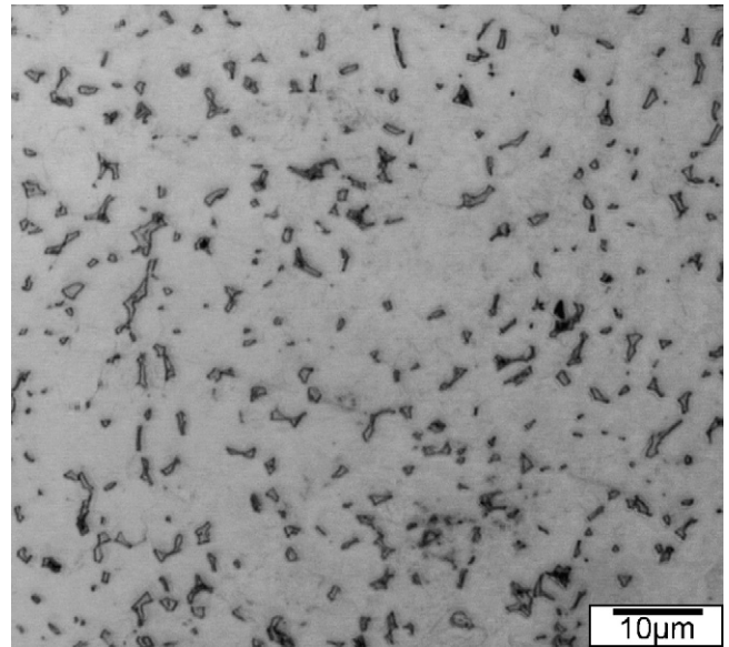
Fig. 3. Light microscopy of reference material (equiaxed microstructure).
