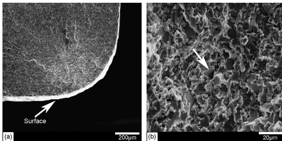
Fig. 13. Fracture surface of reference sample with shot peening: (a) lower magnification and (b) higher magnification of crack initiation location.
