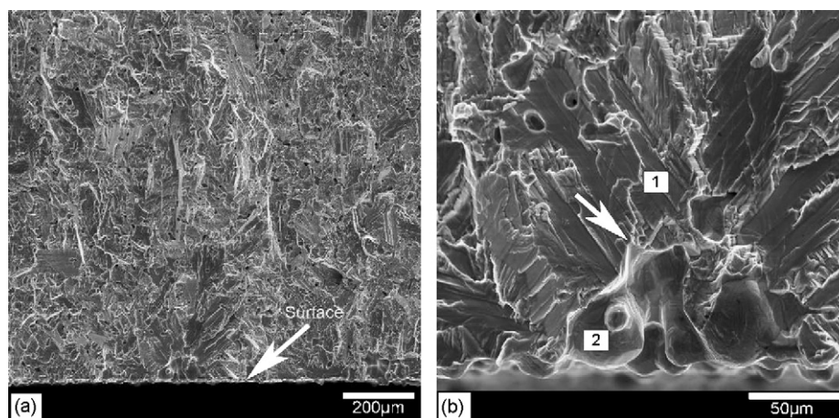
Fig. 8. Fracture surface of MIM sample without shot peening: (a) lower magnification and (b) higher magnification of crack initiation location.
