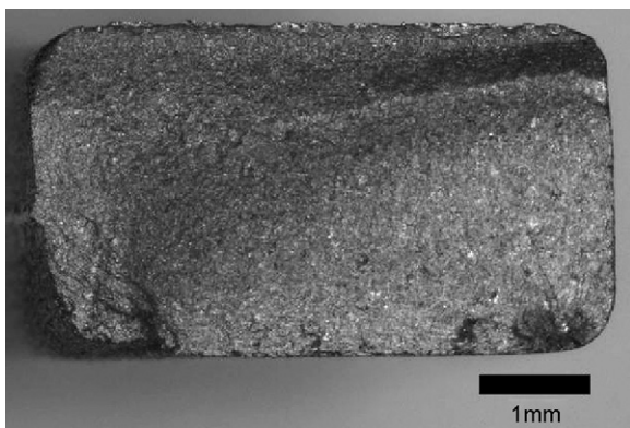
Fig. 12. Typical fracture surface of reference material.
