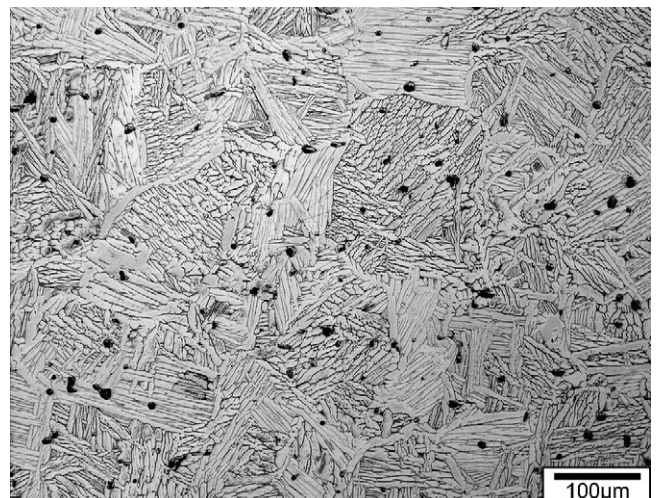
Fig. 4. Light microscopy of MIM sample (fully lamellar microstructure).
