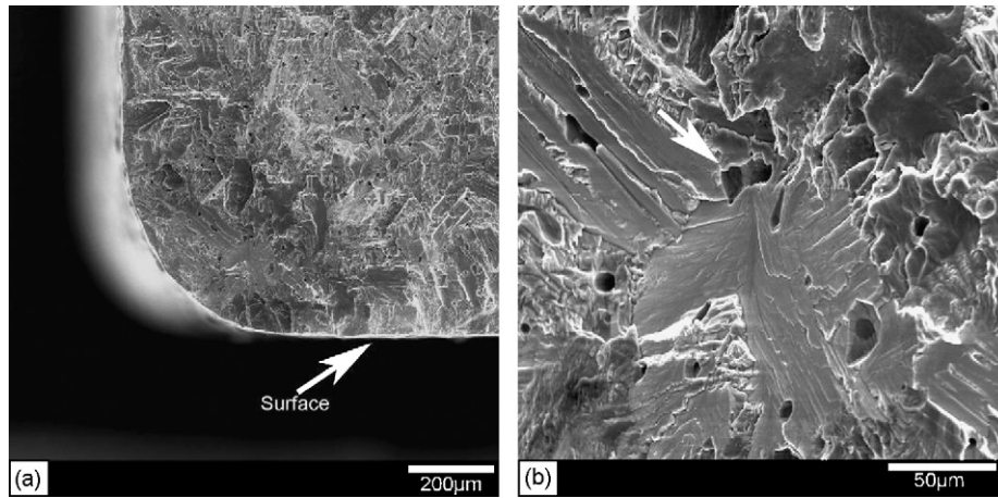
Fig. 10. Fracture surface of MIM sample with shot peening: (a) lower magnification and (b) higher magnification of crack initiation location.
