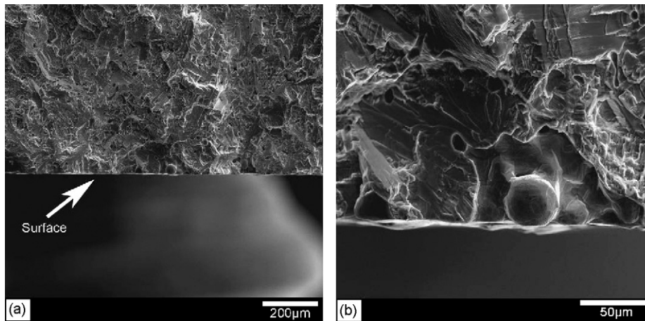
Fig. 11. Typical fracture surface of MIM samples (Fig. 5 with brackets) with shot peening and (a) lower magnification (b) higher magnification of crack initiation location.
