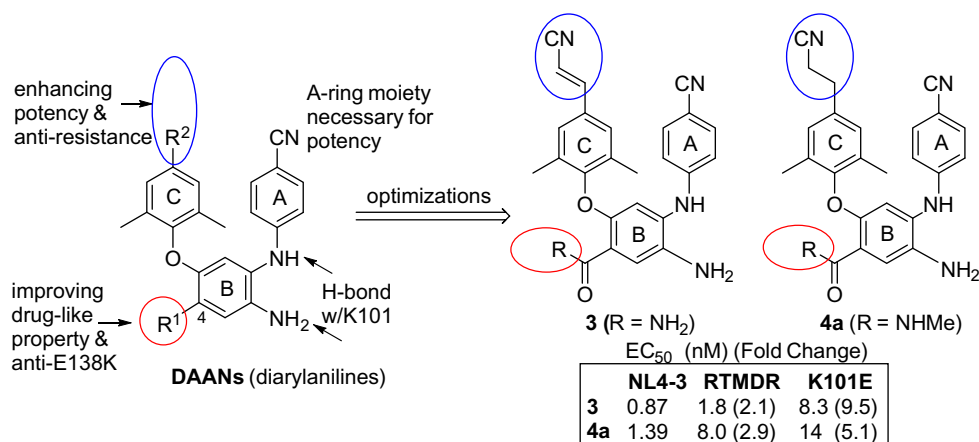
Fig. 2. New-generation NNRTI DAAN leads, known SAR, and leads 3 and 4a .
