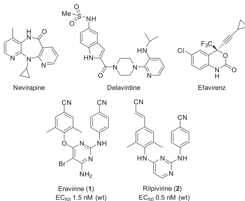
Fig. 1. HIV-1 NNRTI drugs approved by U.S. FDA.
