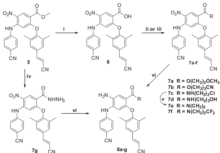
Scheme 1. Reagents and conditions: i. NaOH/MeOH/THF, rt, 2 h; ii. ROH, DCC/DMAP/CH 2 Cl 2 , rt, 2–3 h; iii. a) oxalyl chloride/CH 2 Cl 2 , rt, overnight, b) Et 3 N, amine, rt, 2–3 h; iv. hydrazine/EtOH, reflux; v. K 2 CO 3 /DMF; vi. Zn/AcOH/CH 2 Cl 2 , 0 °C–rt, 1 h.
