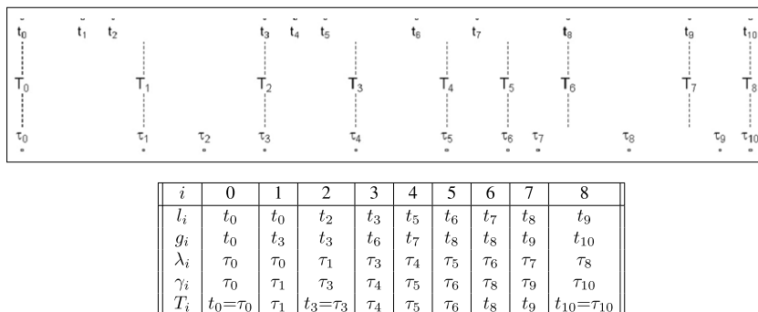
Fig. 2. Example for non-synchronous sampling design with the observation times constructed by the synchronization algorithm and occurring in the estimators and the synchronous approximation.
