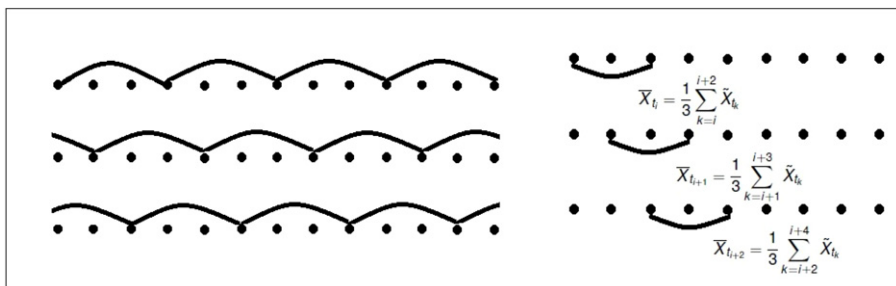
Fig. 1. Sketch of the subsampling approach.
