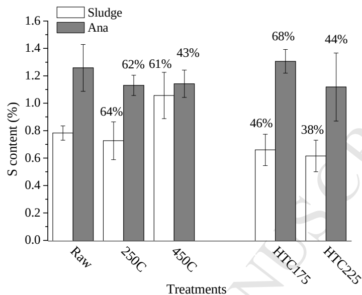
Figure 1. Changes in the total S content in solid samples and S recovery following pyrolysis and HTC treatments. Numbers are S recovery in the solid phase. Error bars of S content represent standard deviation of measurements ( n = 3 ).
