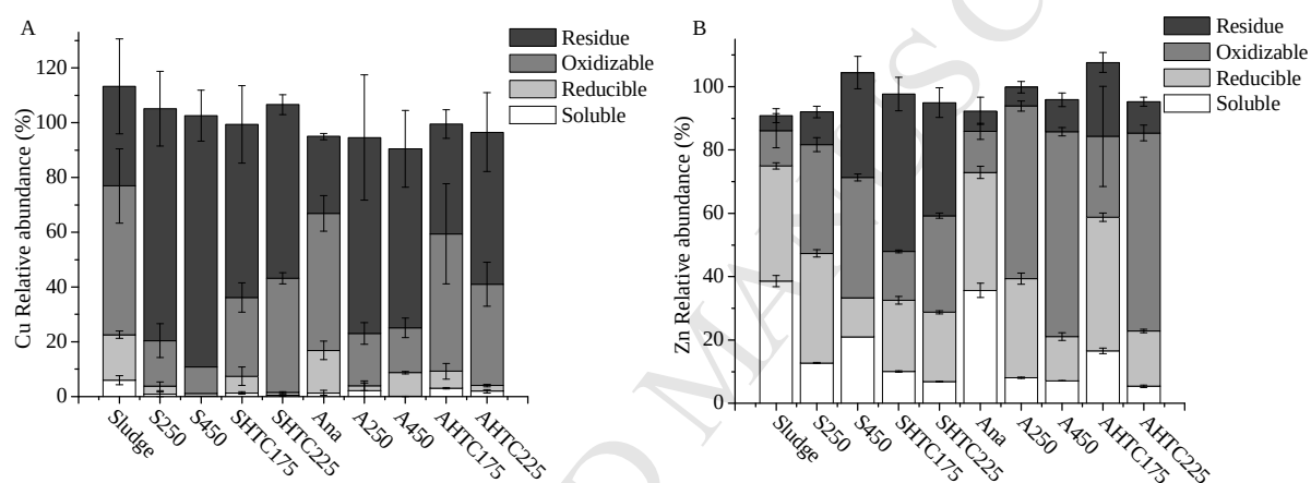
Figure 4. Distribution of Cu (A) and Zn (B) in the aqueous extracts and solid residue during sequential extraction of the raw sludges and their pyrochars and hydrochars. The relative abundance of Cu/Zn in aqueous extract and the solid residue was calculated by Cu/Zn content in the extract/residue divided by total Cu/Zn content in the solid before chemical extraction (determined by ashing and ICP-MS, the raw data were present in Table S3), error bar represents standard deviation of measurements ( n = 3 ).
