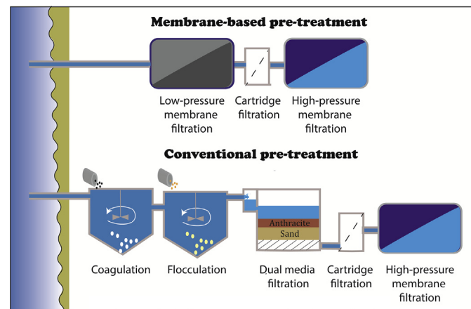
Fig. 3. Schematic diagram illustrating membrane-based and conventional pre-treatment systems for high-pressure membrane filtration.
