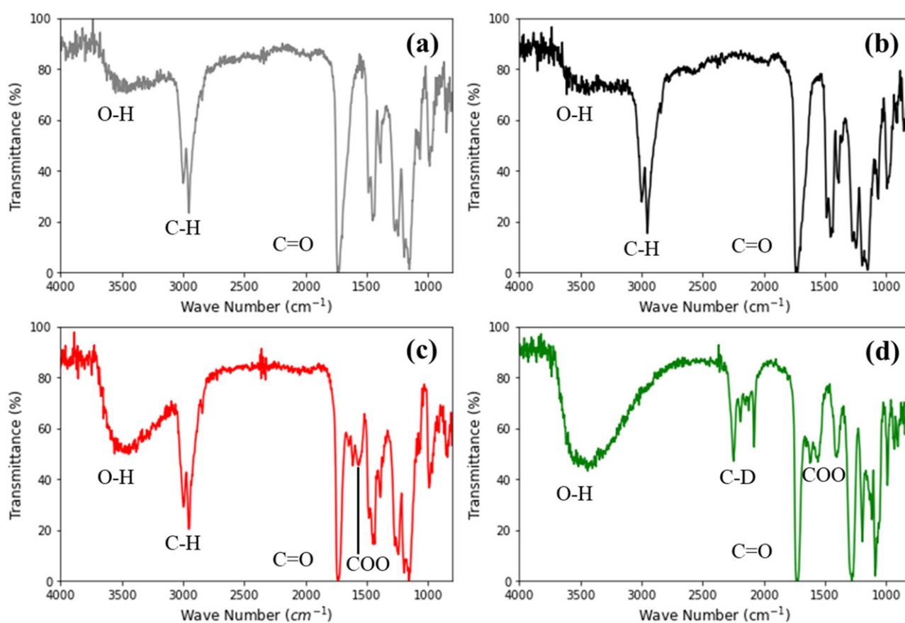
Figure 4. FTIR spectra of (a) hMA-1, (b) hMA-2, (c) Cu-hMA-1 and (d) Cu-dMA-1 thin films.
