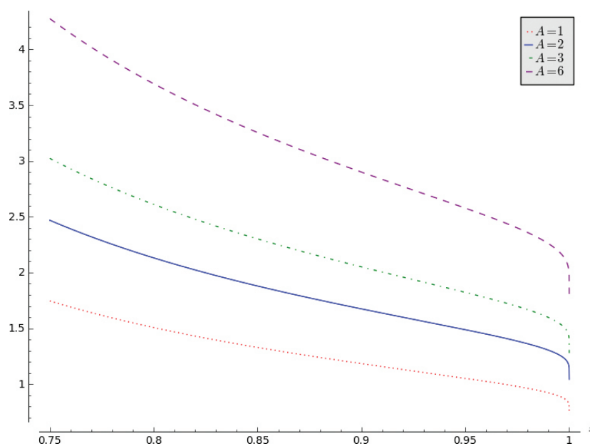
Figure 2. Plots of \sqrt{A \ln(1/(1-x))}/\Phi^{-1}(x) for A = 1, 2, 3 and 6 .
