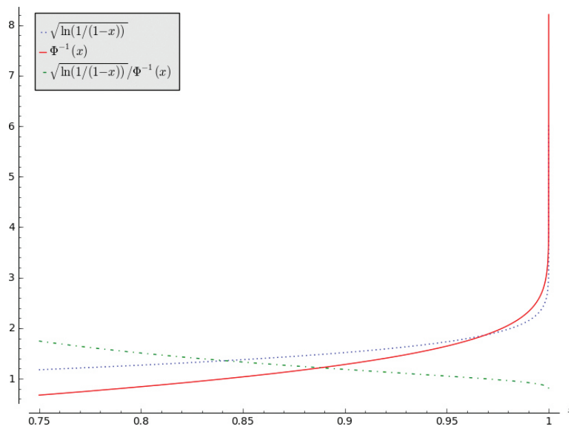
Figure 1. Plots of \Phi^{-1}(x) , \sqrt{\ln(1/(1-x))} and \sqrt{\ln(1/(1-x))}/\Phi^{-1}(x) .
