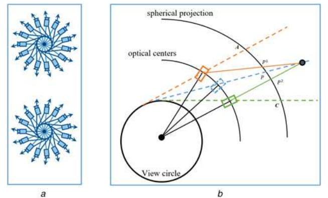
Fig. 7 The virtual ray corresponded to the virtual viewpoint needs to be synthesised a Real rays of the ODS format [2]. In the ODS format, every ray represents the observation in a certain viewpoint b Chunk namely arc section AC in the ODS format. Points A and C are the projections of the real rays, point P needs to be interpolated by some means
