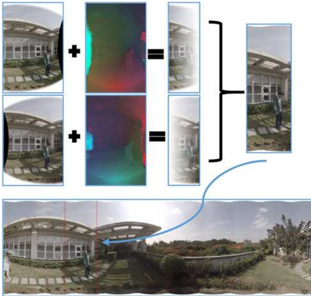
Fig. 8 Process of generating a chunk of the final panorama. We first calculate the pair of optical flow field of the two overlapping region images. Then, we use the optical flow field to warp the original image to get the warped chunks (both the left and the right). Finally, we get the optical flow-based blending chunk. The chunk is part of the final panorama. Every pair of overlapping region images can extract a chunk. We stack all chunks horizontally together to get the final panorama
