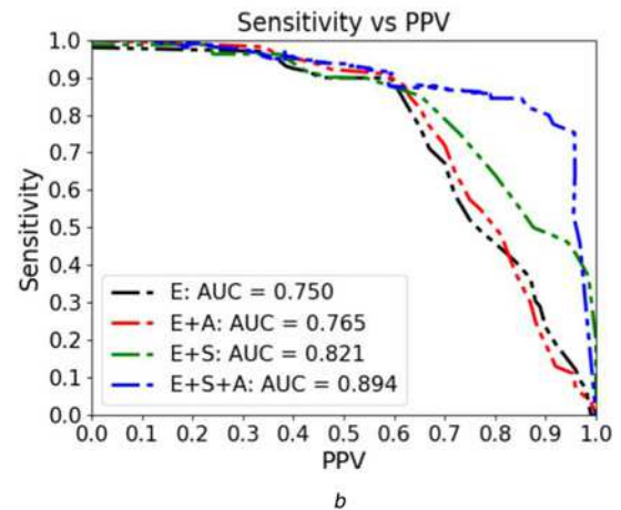
Fig. 10 Performance of deep neural net (SN versus PPV) for HE detection
