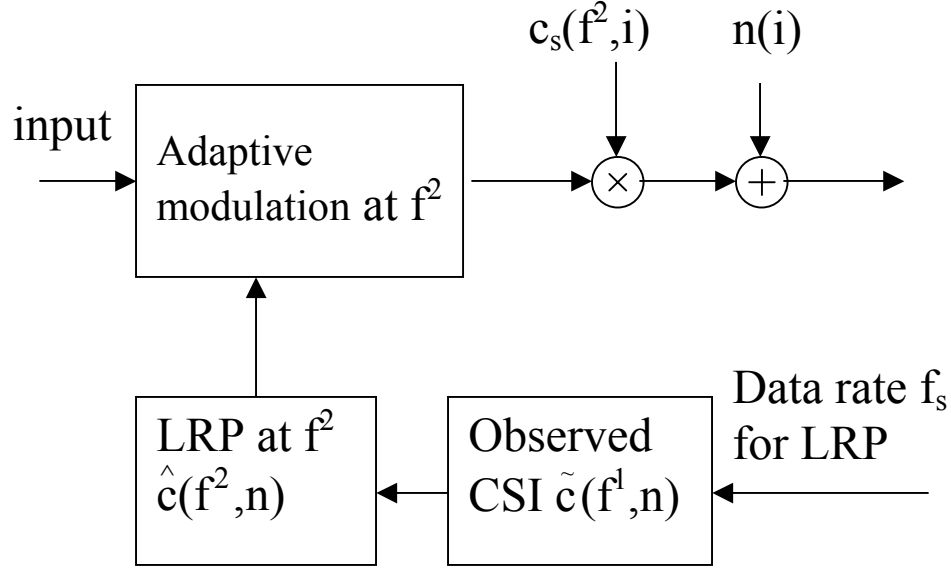
Figure 4.1 System model of adaptive modulation at carrier f^2 based on the channel observations at f^l .
