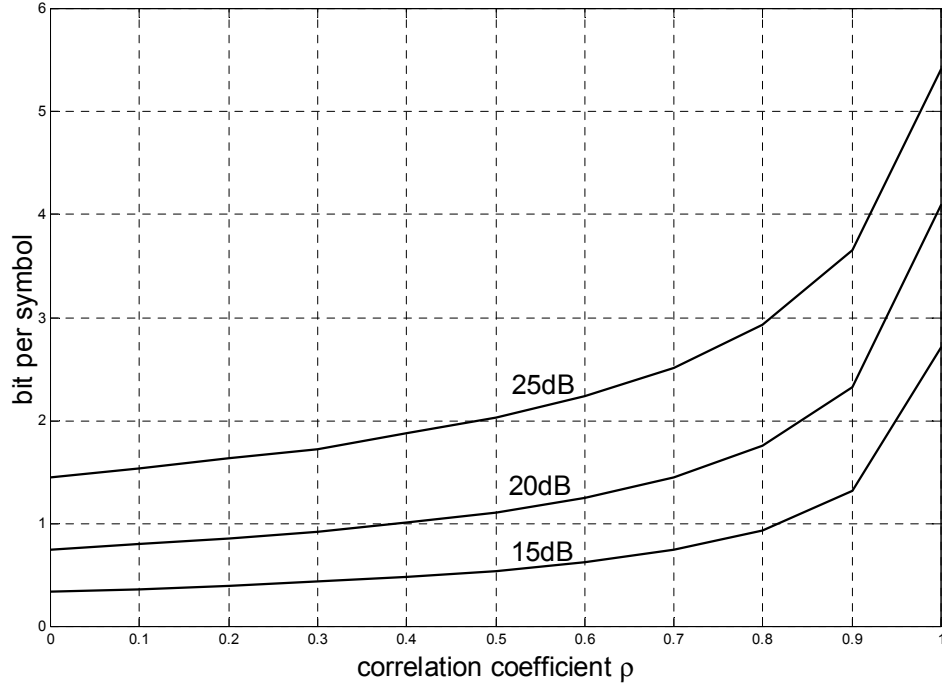
Figure 3.9 Bit per symbol vs. \rho for different \text{SNR} = S_{\text{avg}}/N_0 for power control M-QAM. Target \text{BER}=10^{-3} .
