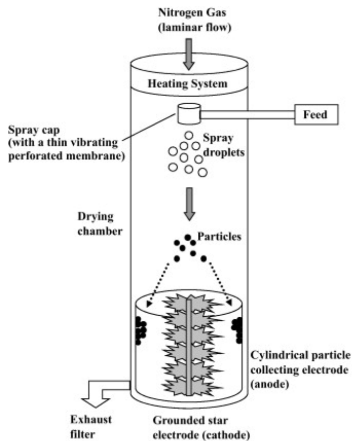
FIGURE 2 - Schematic of spray drying process (Lee et al., 2011)
