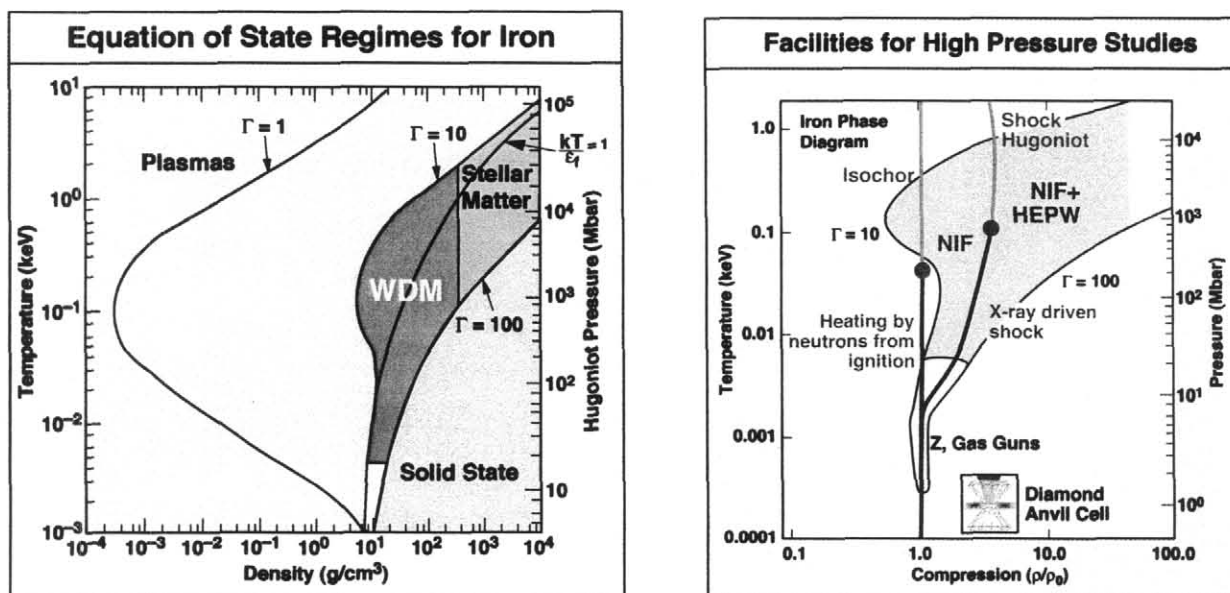
Fig. 2a, left, shows the phase space for iron with the warm dense matter (WDM) phase highlighted. The lines labeled with \Gamma referring to the strength of coupling between ions, with higher \Gamma being strongly coupled. Also shown is the approximate location of electron degeneracy kT/\epsilon_F = 1 . Fig. 3b, right, details NIF's ability to reach high pressures using long pulse NIF, NIF plus HEPW and NIF ignition neutrons to isochorically heat materials to off-Hugoniot conditions. Other facilities such as z-pinch, gas gun, and diamond anvil cells are shown for comparison.
