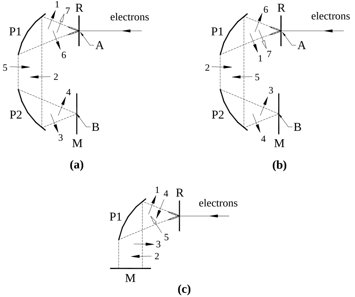
Figure 7.3: Radiation polarization in the cavity as the radiation travels through all components: (a) the upper half of the radiation cone and (b) the lower half of the radiation cone. The numbers indicate chronological events. For example, the polarization marked number 1 is the polarization of the transition radiation just emitted from electrons and the polarization marked number 7 (shown by an unfilled head arrow) is the radiation after one circulation in the cavity. The diagram in (c) shows a setup that does not meet the required polarization condition.
