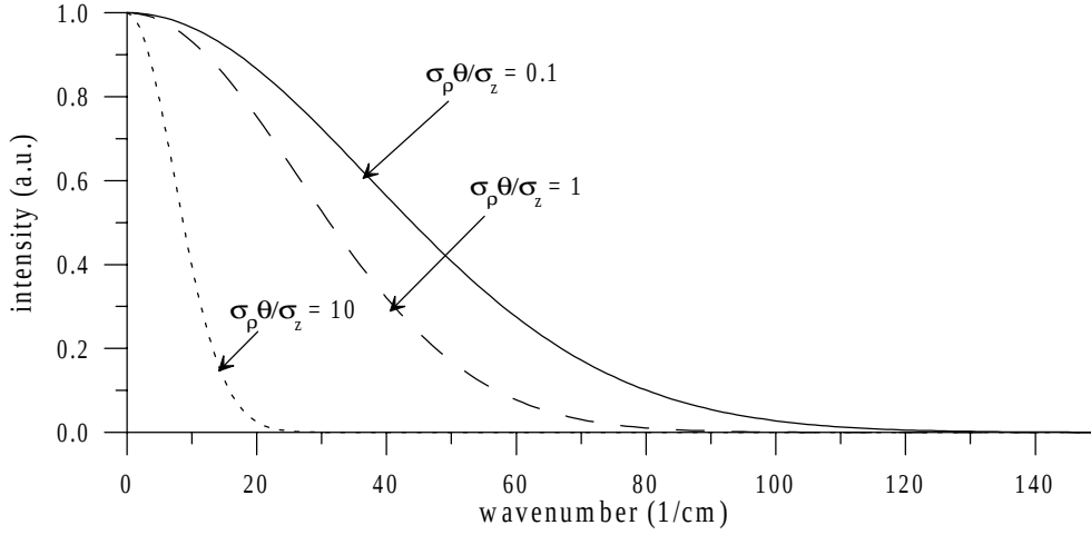
Figure 4.16: Coherent radiation spectral distribution for \sigma_p \theta / \sigma_z = 0.1 (solid), 1 (dashed-line), and 10 (dotted-line).
