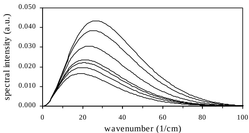
Figure 4.14: Calculated spectral intensity of coherent transition radiation from a Gaussian bunch with \sigma_\rho = \sigma_{\rho,\text{CENTER}} .
