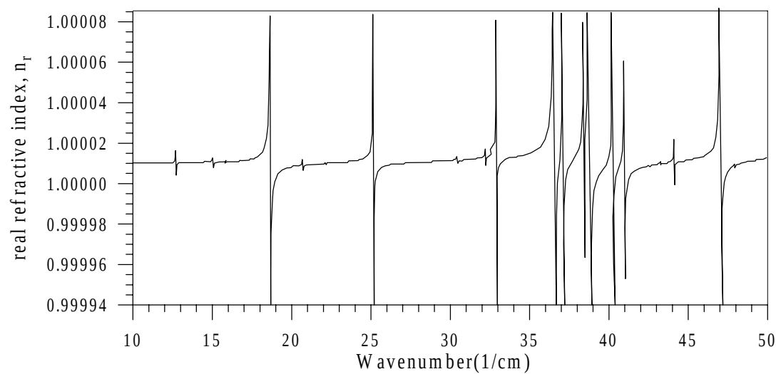
Figure 5.11: The real refractive index of air at room temperature and 1.5 Torr partial pressure [29] for the spectral range 10-50 \text{cm}^{-1} wavenumber.
