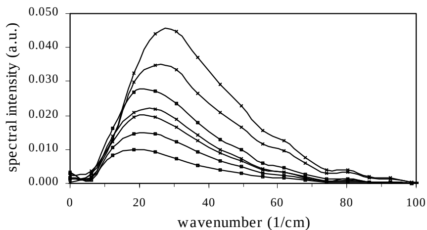
Figure 4.13: Spectral intensity of coherent transition radiation from the bunch with various beam sizes.
