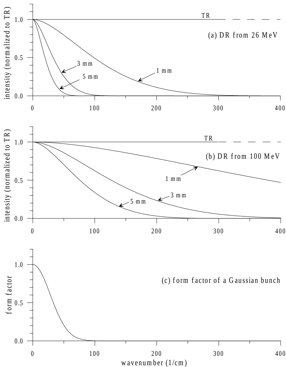
Figure 6.9: Spectral distribution of diffraction radiation generated by different aperture sizes for (a) 26 MeV beam and (b) 100 MeV beam. The form factor of a Gaussian bunch with \sigma_z = 40 \mu\text{m} is shown in (c).
