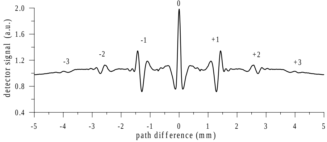
Figure 5.6: The interferogram showing multiple reflections in the pyroelectric sensor.
