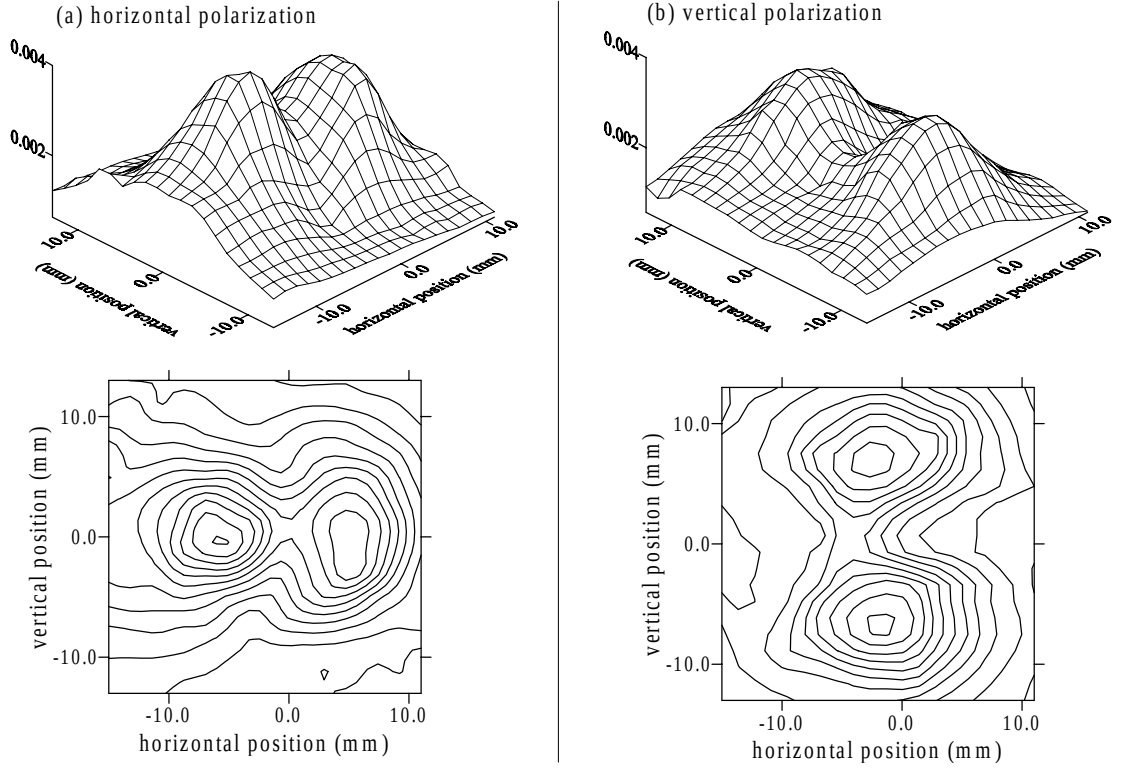
Figure 4.11: Horizontally and vertically polarized radiation components measured using a wire grid polarizer.
