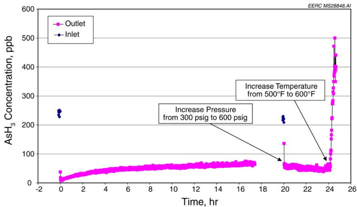
Figure 27. Breakthrough curve for the Corning-treated monolith with Catalyst 2 additive for the control of \text{AsH}_3 at various pressures and temperatures.
