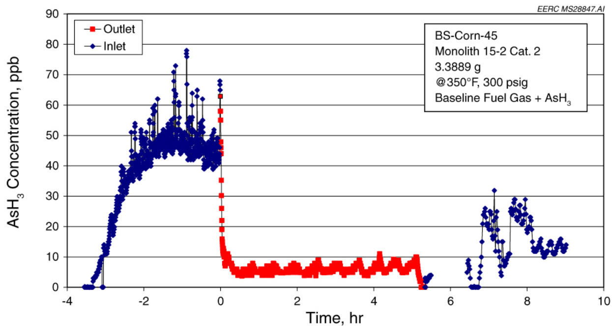
Figure 26. Breakthrough curve for Corning-treated carbon monolith with Catalyst 2 additive for \text{AsH}_3 control.
