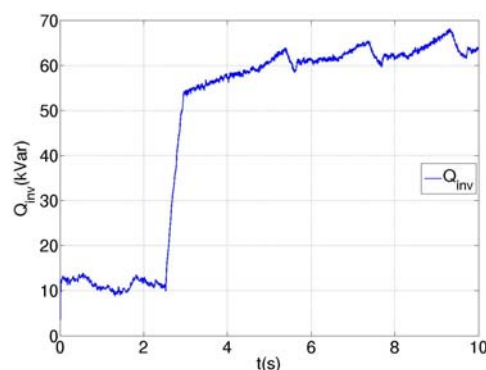
(d) Inverter reactive power (kVAR) before and after load change.
