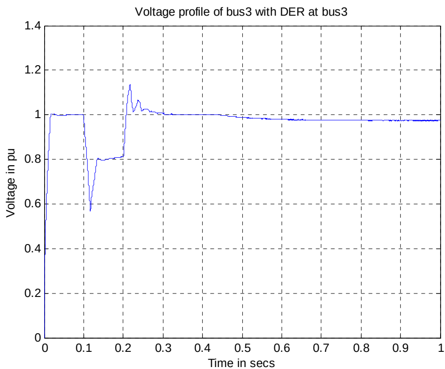
Figure 11-16. Voltage profile at bus3 with DER.
