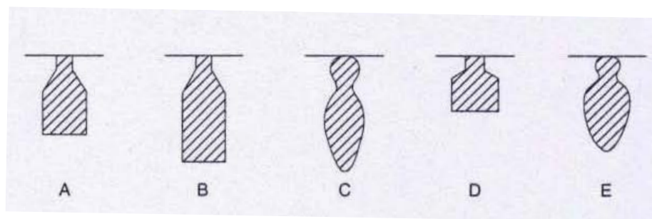
Figure 4-4. NEMA induction motor rotor bar designs. c
