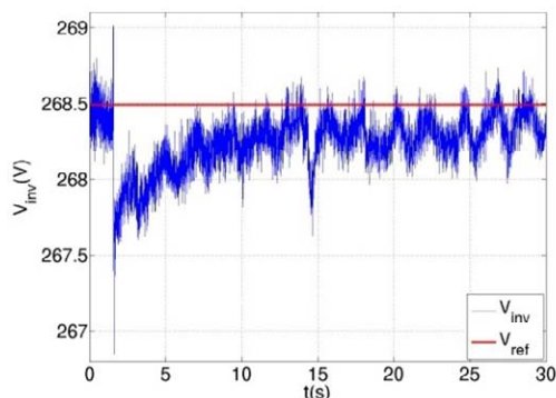
(c) PCC rms voltage with voltage regulation (V).
