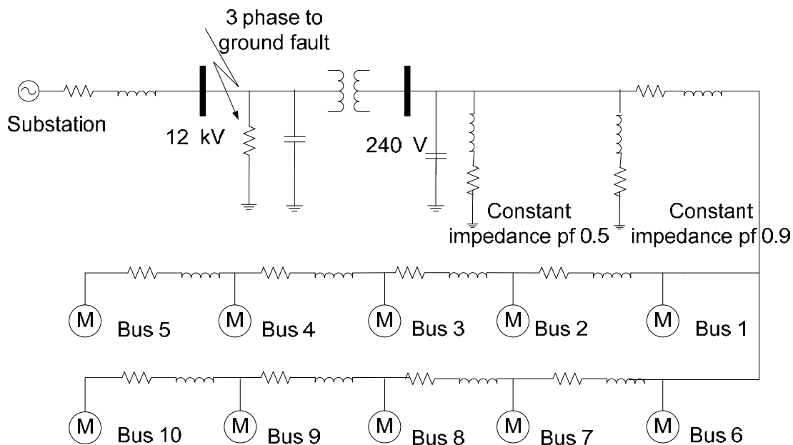
Figure 11-5. System configuration with 50kVA motor loads.
