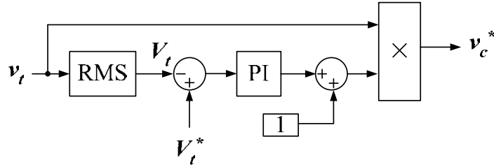
Figure 8-2. Controller diagram.
