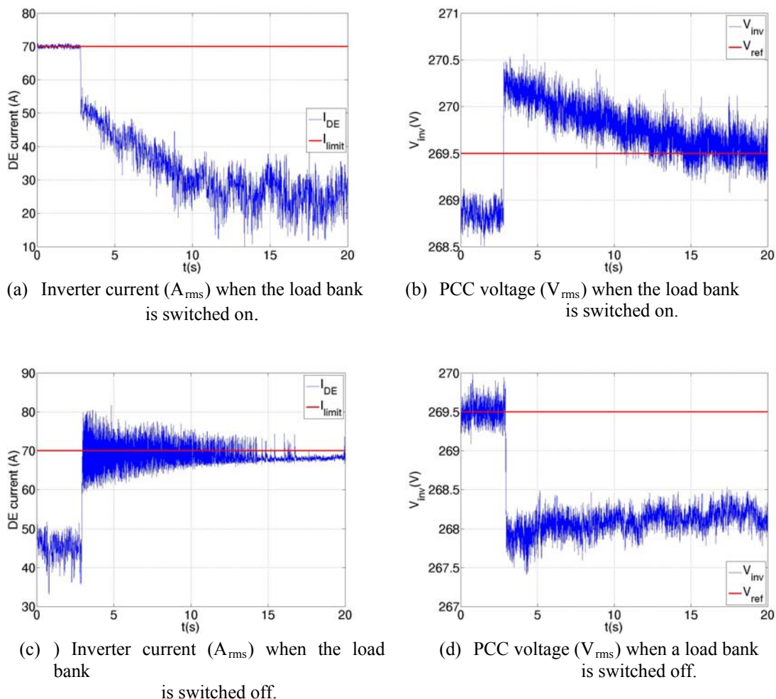
Figure 10-14. Testing results of current limit for voltage regulation controller.
