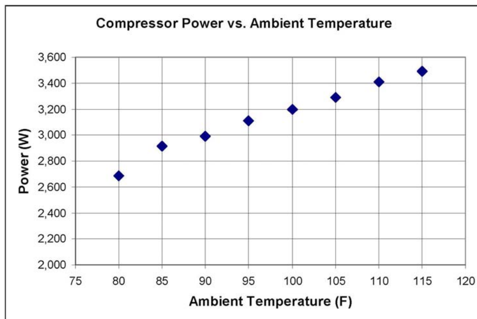
Figure 3-1. Increase in running power (steady-state) of single-phase A/C compressor motor with increasing temperature for the SEER 10 to 13 units of reference [5]. b
