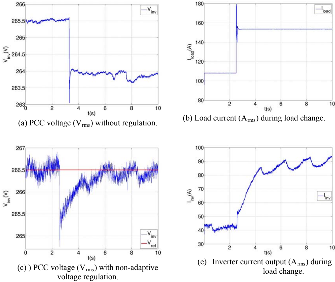
Figure 10-16. Testing results of voltage regulation for load change.
