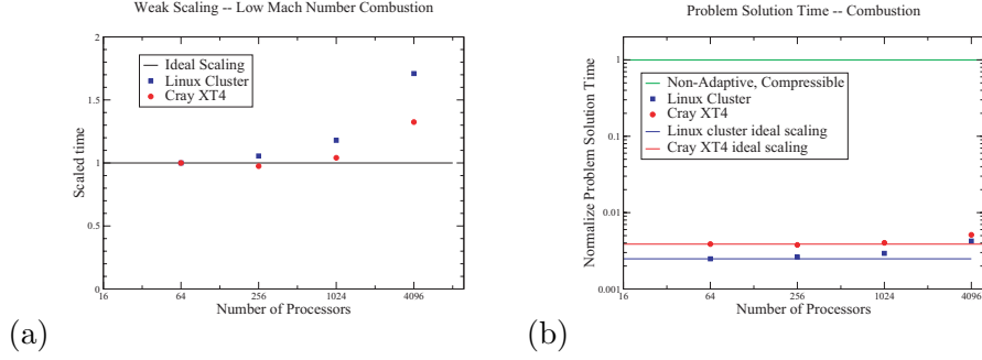
Figure 1. Parallel performance of the low Mach number adaptive algorithm: (a) Weak scaling behavior of the adaptive low Mach number algorithm. (b) Scaling of time-to-solution, relative to a compressible solver.
