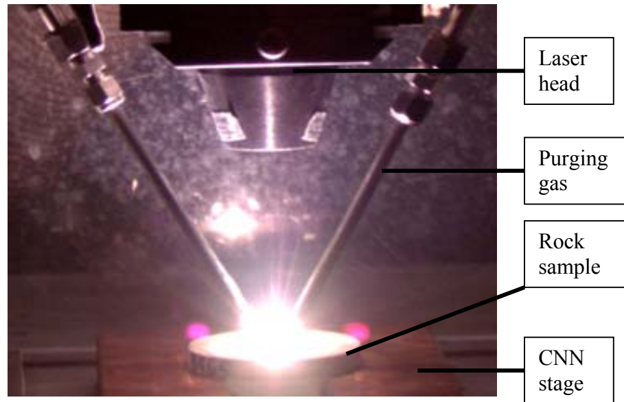
Figure 2 Photograph of the laser rock drilling system
