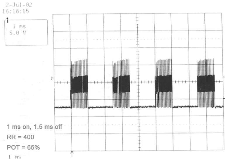
Figure 1 Waveforms of an electrically-pulsed CO 2 laser beam.
