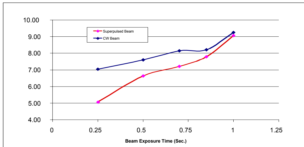
Figure 7 Comparison of specific energy as a function of beam exposure time for CW and SPP CO 2 laser beam rock drilling.
