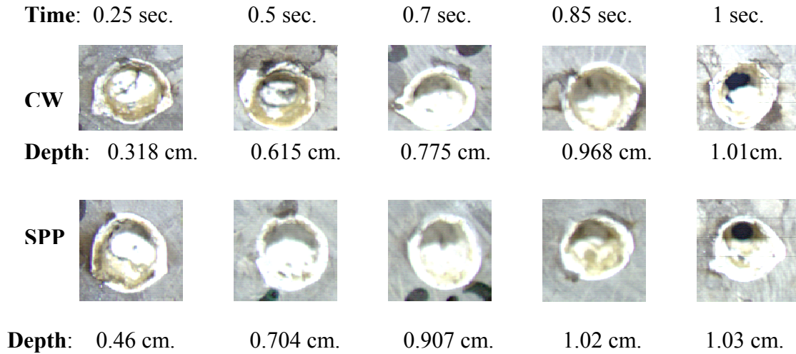
Figure 6. Top view of holes drilled with different beam exposure time and laser operation modes. The hole diameter is 6.3 mm.
