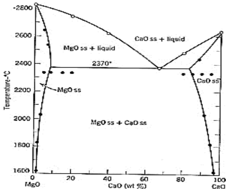
Figure 8 Phase equilibrium diagram for system CaO-MgO. Solid circles are data points of solid solution, and open circles represent liquidus points.
