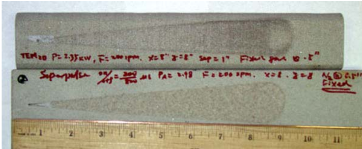
Figure 5. Comparison of linear tracks produced by CW beam (top) and superpulsed pulse beam (bottom) showing similar surface characteristics.
