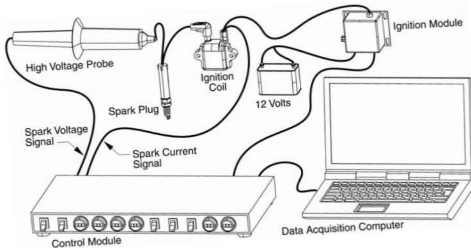
Figure 2. Programmable Ignition System
