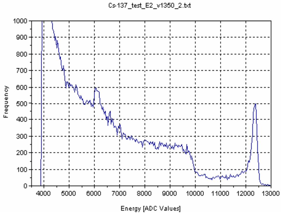
Fig. 16: The pulse height spectra with 137 Cs from the 4 x 4mm 2 x L=6mm CdZnTe Frisch collar detectors fabricated from Digirad growth materials (a) with standard NIM system and 142A preamplifier (b) the primary test with RENA3 chips package (note that the energy lines are not calibrated).
