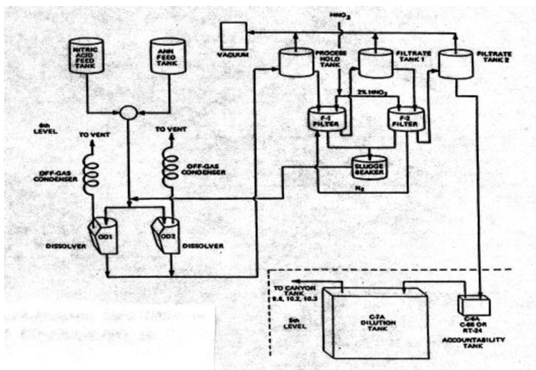
Figure 11 – Special Recovery Flow Diagram; Oxide Dissolution Process
