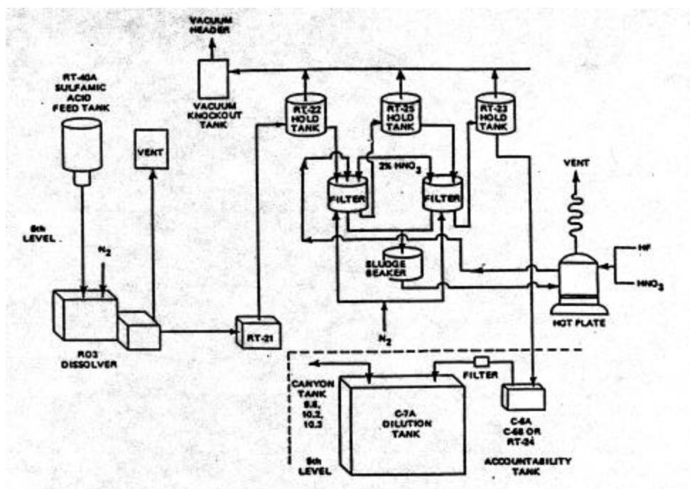
Figure 10 – Special Recovery Flow Diagram; Metal Dissolution Process
