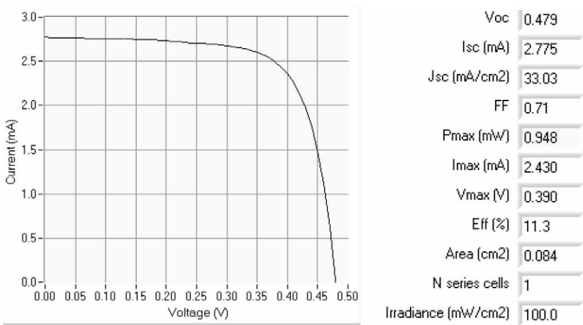
Figure 7. I-V curve of a CIGS solar cell produced in the large area reduction and selenization furnaces. Sample is tested under AM1.5 illumination.
