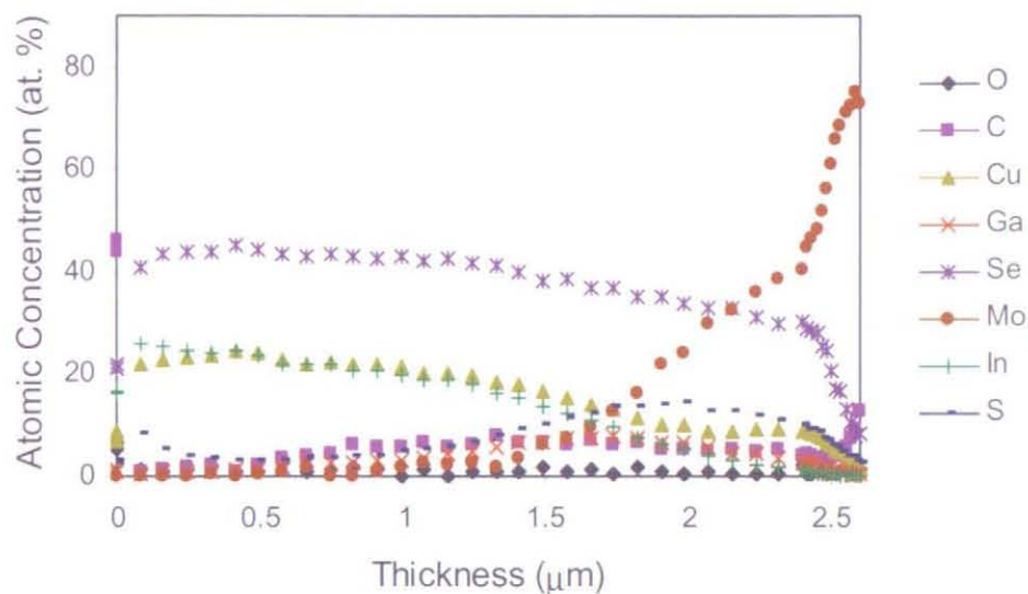
Figure 1. SIMS Depth profile of a CIGS Absorber layer using ISET's ink-based processing scheme involving selenization of nanoparticle precursors.
