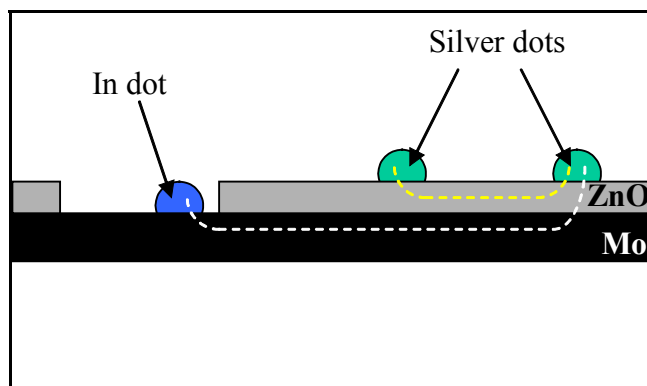
Figure 10. Schematic of a ‘dot test’ for evaluation of contact resistance between the ink and the ZnO layer.
