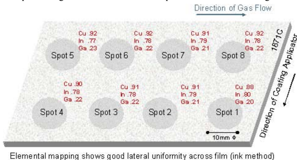
Figure 4. XRF Elemental analysis mapping of a reduced alloy film
