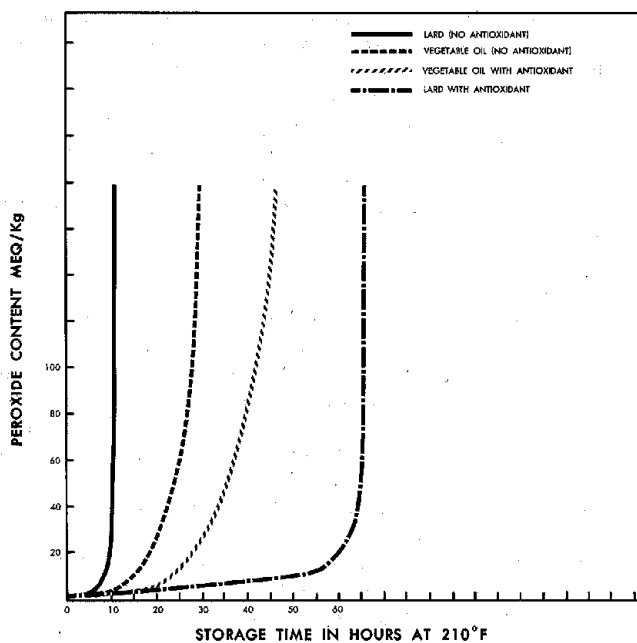
Fig. 7. Peroxide content versus storage time of some typical fats.
