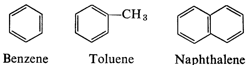
Figure 13. Aromatic molecules
