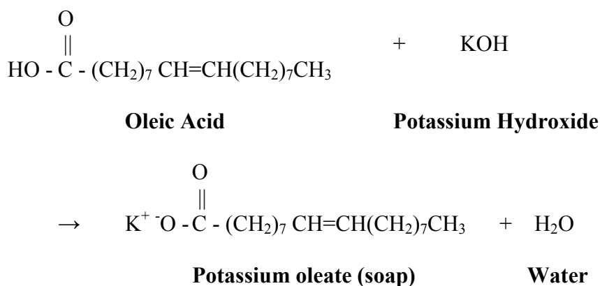
Figure 7. Formation of Soap
