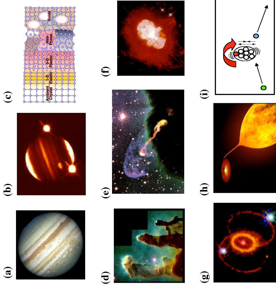
Fig. 2. HED facilities open up a unique experimental window into the physics of the universe. (a) planetary interiors, (b) hypervelocity impacts, (c) ultrafast lattice dynamics, (d) radiatively driven molecular clouds, (e) protostellar jets, (f) stellar dynamics, (g) core-collapse supernovae, and supernova remnants, (h) accreting black holes and neutron stars, and (i) excited state nuclear reactions in ignition experiments.
