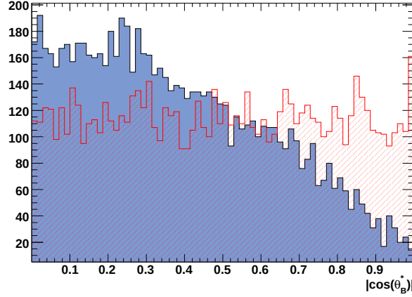
Figure 5.3: Monte Carlo comparison of |\cos(\theta_B^*)| for signal (solid blue) and continuum background (hatched red). The histograms are normalized to equal areas.
