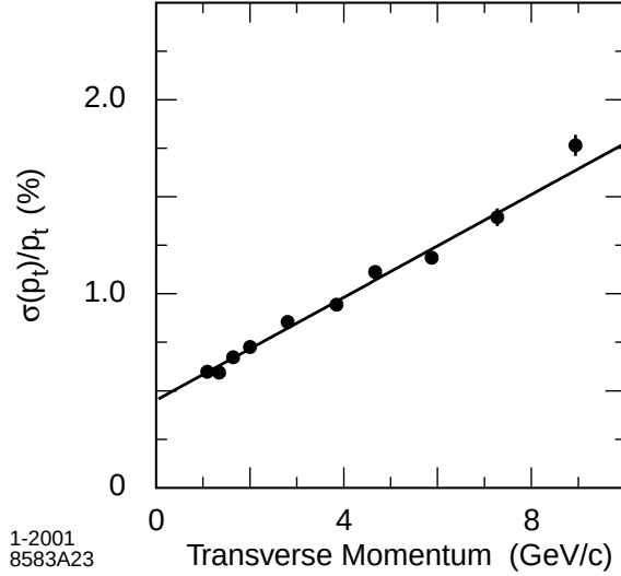
Figure 4.3: Resolution of transverse momentum of cosmic ray muons as a function of transverse momentum.
