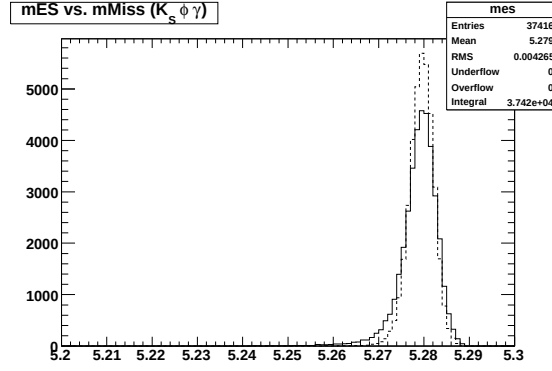
Figure 5.1: Comparison of m_{\text{ES}} (solid) and (m_{\text{Miss}} + m_B)/2 (dashed) for B \rightarrow K\phi\gamma . The vertical scale is arbitrary, though both histograms are normalized to the same area.
