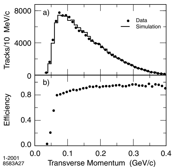
Figure 4.5: SVT low-momentum track reconstruction performance. The top plot (a) shows the soft pion momentum from D^{*+} \rightarrow D^0 \pi^+ in B\bar{B} data (after background subtraction) compared to B\bar{B} Monte Carlo simulation. The bottom plot (b) shows the Monte Carlo reconstruction efficiency of the soft pion.
