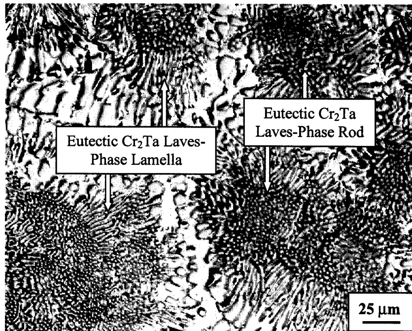
Figure 2 Cross-sectional microstructure of the directionally-solidified Cr-9.25 at.% Ta alloy
