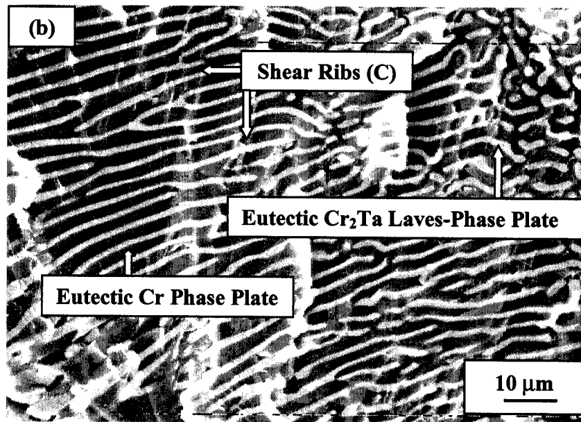
Figure 3 Fracture surfaces of the drop-cast (a) and directionally-solidified (b) Cr-9.25 at.% Ta alloy tensile-tested at room temperature
