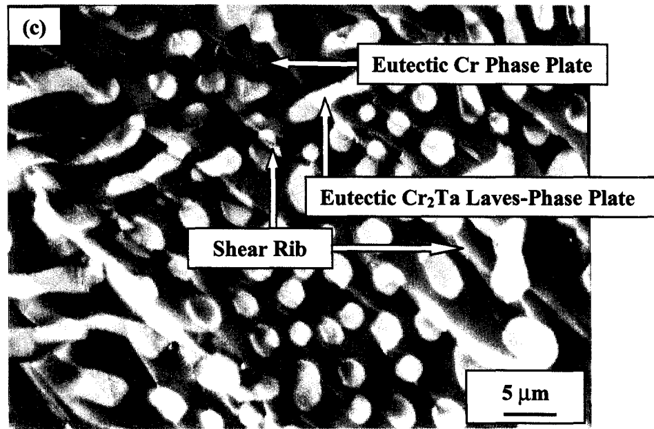
Figure 6 Fracture surfaces of the drop-cast (a) and directionally-solidified (b and c) Cr-9.25 at.% Ta alloy tested for fracture toughness
