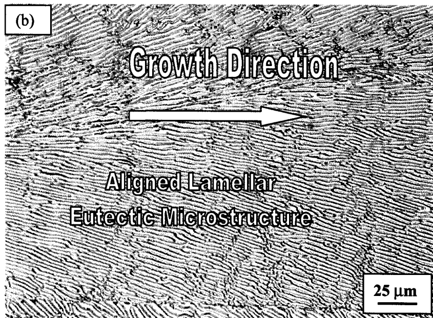
Figure 1 Microstructures of the drop-cast (a) and directionally-solidified (b) Cr-9.25 at.% Ta alloy along the longitudinal direction of the ingots
