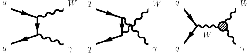
Figure 3: ISR and s -channel diagrams for W\gamma production. The FSR diagram is not shown.
