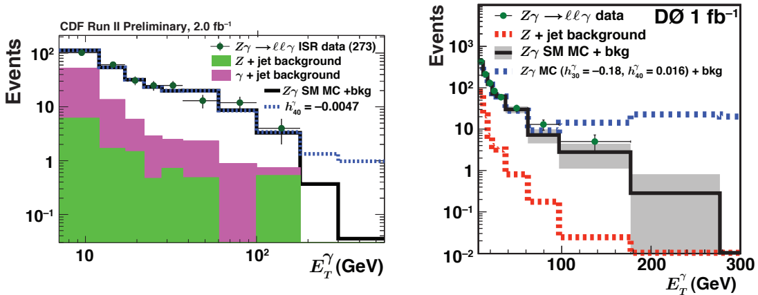
Figure 2: Photon E_T spectra in Z\gamma production for the CDF and D0 analyses respectively.
