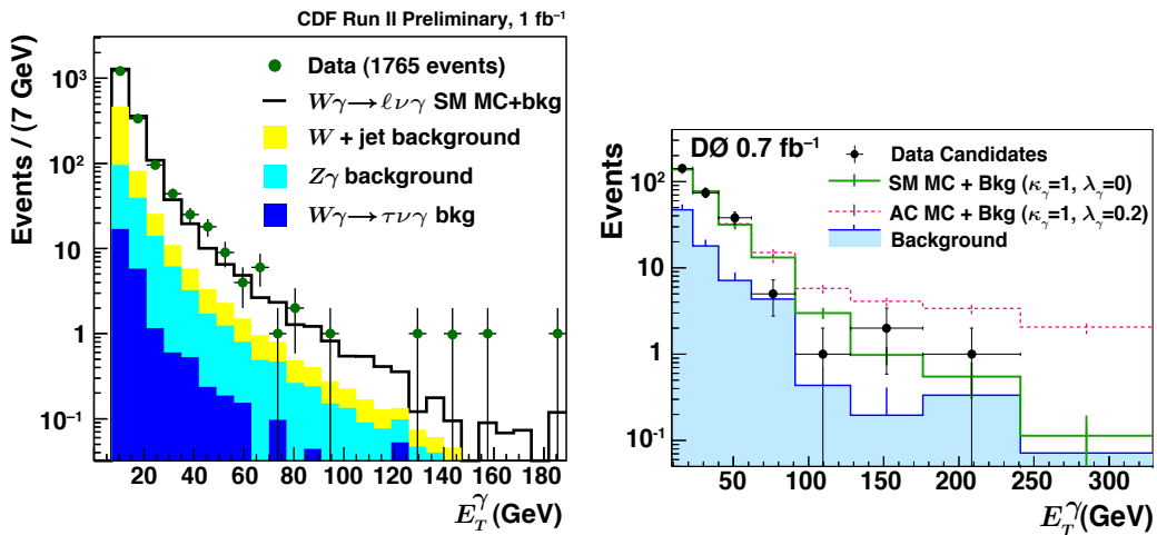
Figure 4: Photon E_T spectra for the CDF and DØ W\gamma analyses respectively.
