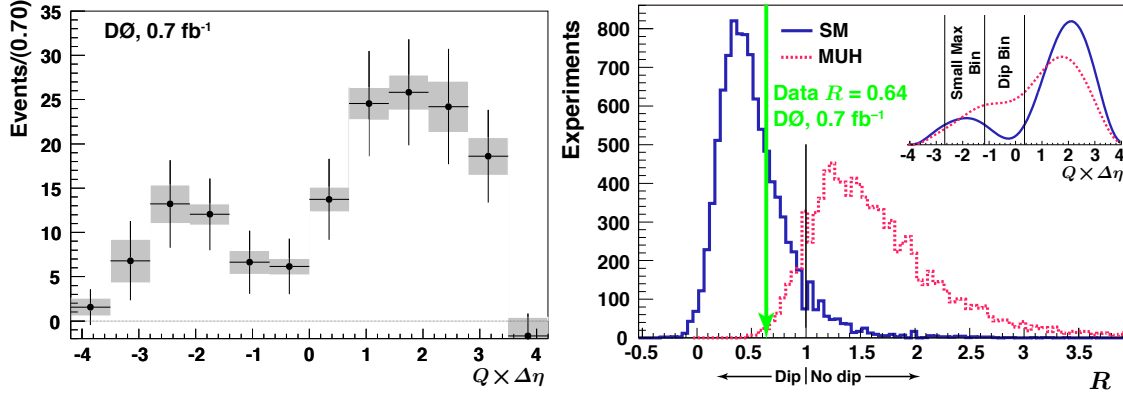
Figure 5: Q_\ell \times \Delta\eta distribution (left) and its analysis (right).
