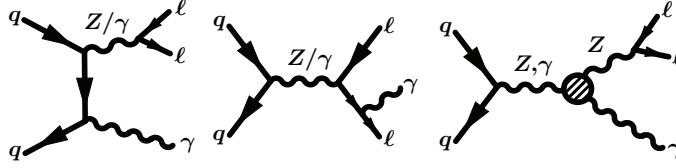
Figure 1: Diagrams for Z\gamma production: ISR, FSR and the forbidden s -channel involving the trilinear gauge coupling.
