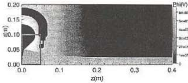
Figure 3: Snapshot of the particle distribution (dark yellow) at the end of a HCX source simulation. Color contour plot of the electrostatic potential are rendered in vacuum areas (Black areas represent conductors). The red box sets the limits of the mesh refinement patch that has been used in one of the runs.
