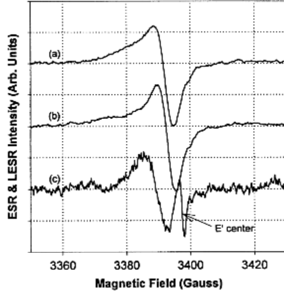
Fig. 3. ESR and LESR spectra of a-SiS x :H. The LESR spectra [(a) and (b)] were measured at 40 K with 8 μW of microwave power. (a) 2 at. % of sulfur and (b) 0.6 at. % of sulfur. The ESR spectrum (c) was measured at room temperature with 20 μW of microwave power for the sample with 0.6 at. % of sulfur.
