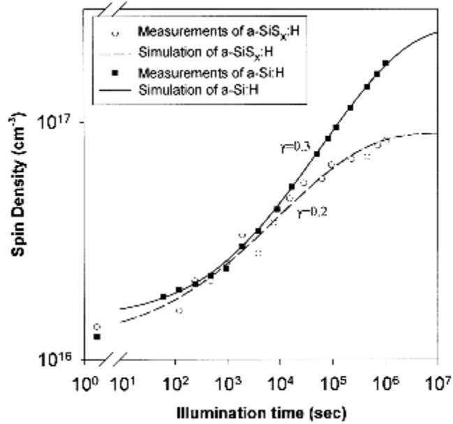
Fig. 4. Kinetics of light-induced defect generation for undoped a-Si:H and a-SiS x :H ( x = 6 \times 10^{-3} ). The smooth lines are fits to the experimental data (symbols) with Eq. (1) with the parameters: N_0 = 1.2 \times 10^{16} \text{ cm}^{-3} , N_S = 9 \times 10^{16} \text{ cm}^{-3} , \tau_g = 8 \times 10^4 \text{ s} and \beta = 0.38 for a-SiS x :H ( x = 6 \times 10^{-3} ); N_0 = 1.5 \times 10^{16} \text{ cm}^{-3} , N_S = 2.5 \times 10^{17} \text{ cm}^{-3} , \tau_g = 8 \times 10^5 \text{ s} and \beta = 0.45 for a-Si:H
