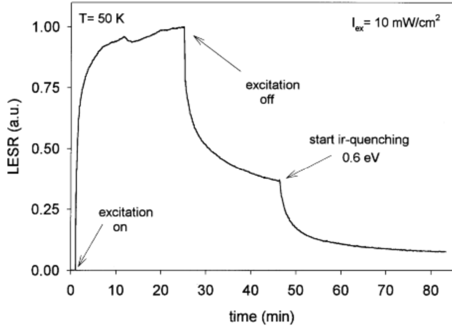
Fig. 12. Infrared quenching of residual LESR. The data up to approximately 45 min show the rise and decay of the LESR signal after the excitation source has been turned on and off, respectively. Infrared quenching is initiated after approximately 45 min with an infrared cut-off energy of 0.6 eV.
