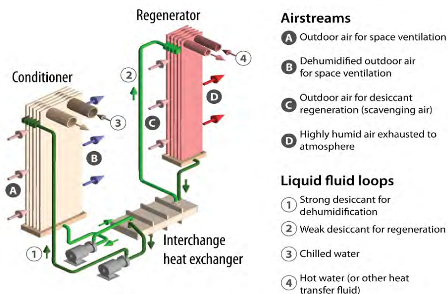
Figure 2–1. Core components of a low-flow LDAC.
