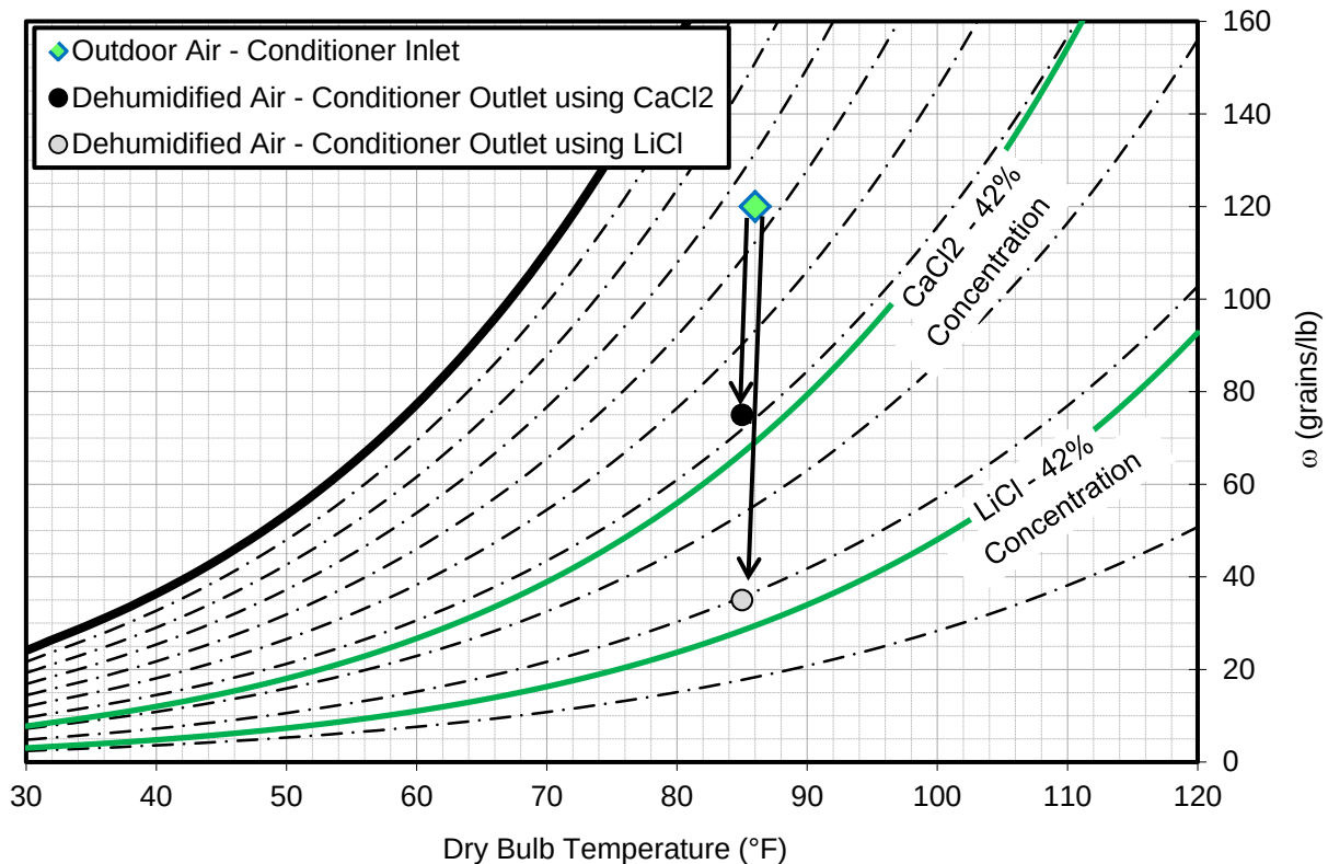
Figure 4–1. Examples of conditioner inlet and outlet air conditions using different desiccants.
