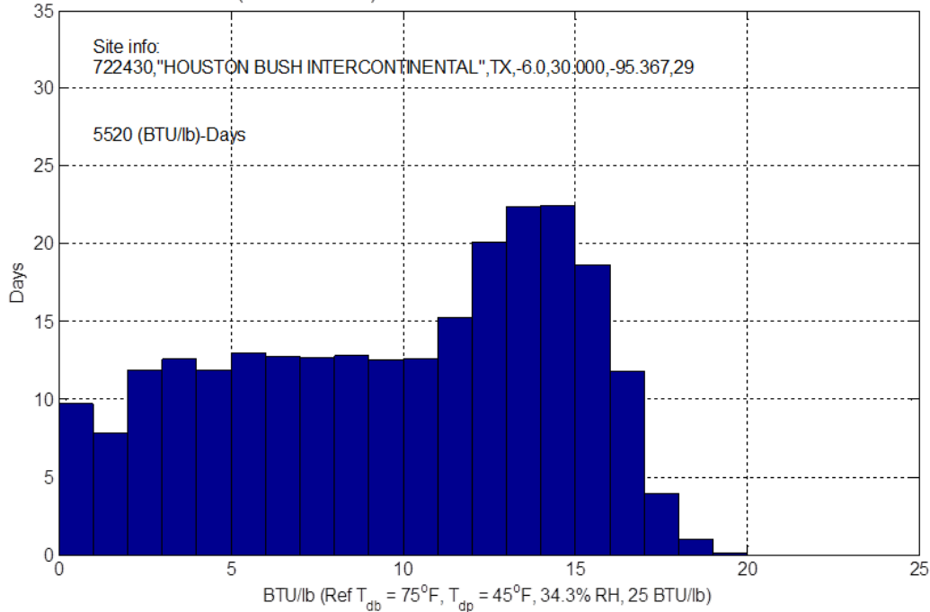
Figure 3-3. Total ventilation load bins for Houston.
