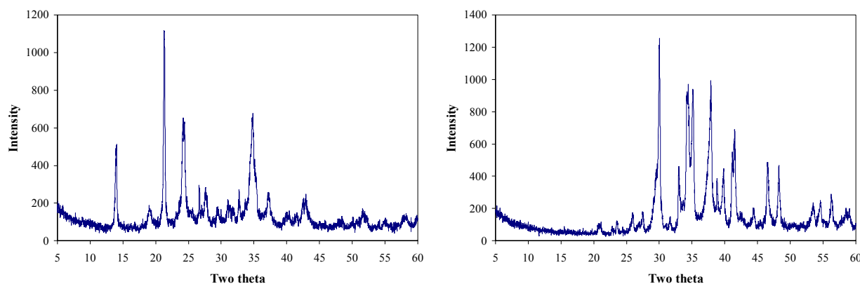
Figure 6b. Calcine made with metakaolinite. Zeolite present is hydroxysodalite. Figure 6c. Calcine made without metakaolinite. Phase present is sodium carbonate.
