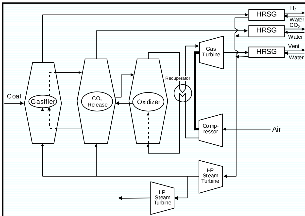
Figure 7. Process flow diagram incorporating the AGC module with other unit operations.
