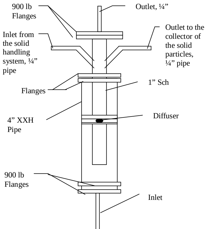
Figure 6. Lab-scale reactor design.
