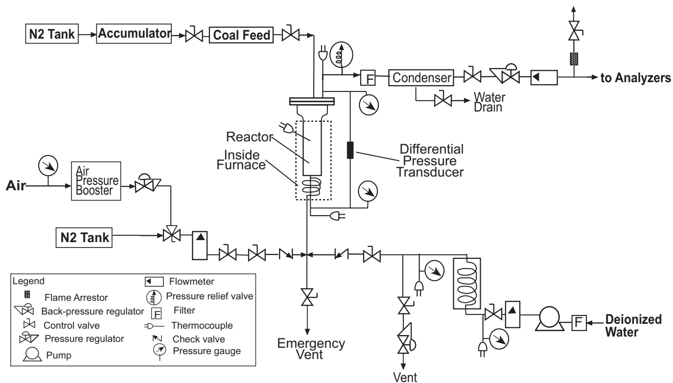
Figure 2. Bench-scale system process and instrumentation diagram.
