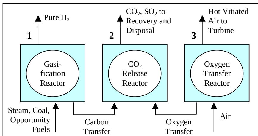
Figure 1. Conceptual design of the AGC technology.
