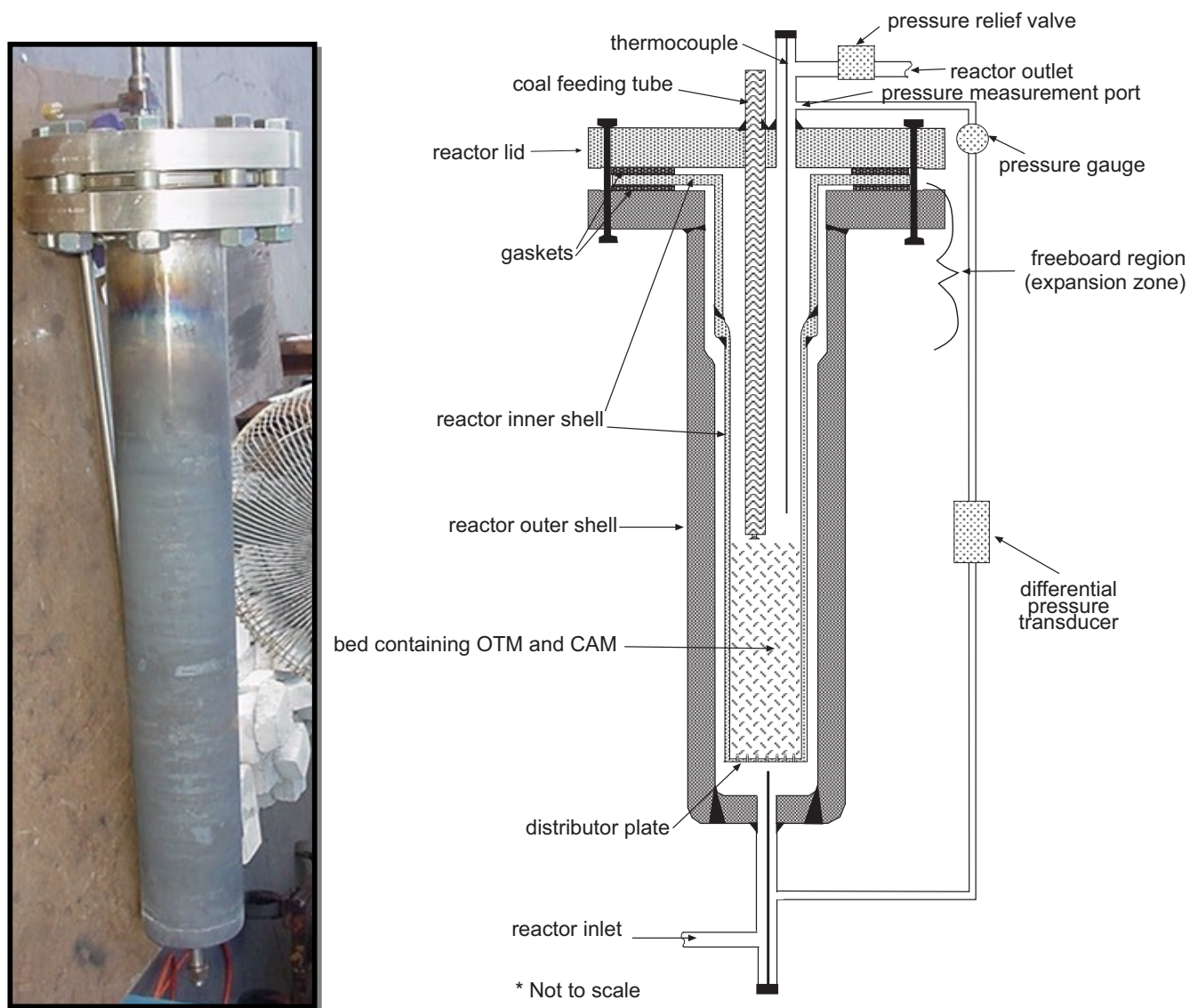
Figure 3. Bench-scale reactor photo and diagram.
