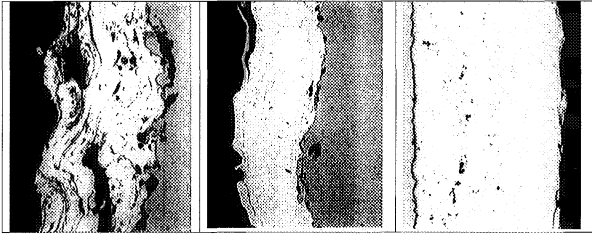
Figure 6 Bead-blasted surfaces of thermal-deposited Al. (a) 0.005" diameter beads applied at 100 psi on Twin wire arc Al showed little densification; (b) 0.015" diameter beads applied at 60 psi on Twin wire arc Al reduced the coating porosity; (c) 0.002" diameter beads applied on HVOF Al.
