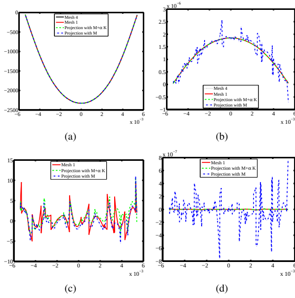
Fig. 3. (a) The electric fields computed with direct finite-element simulation using Mesh 1 and 4 and the electric fields projected from Mesh 1 to Mesh 4. (b) The magnetic fields. (c) The errors of the electric fields. (d) The errors of the magnetic fields.
