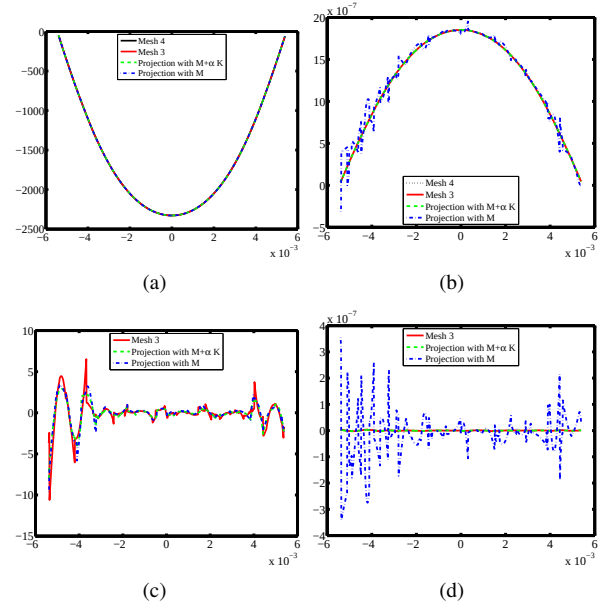
Fig. 5. (a) The electric fields computed with direct finite-element simulation using Mesh 3 and 4 and the electric fields projected from Mesh 3 to Mesh 4. (b) The magnetic fields. (c) The errors of the electric fields. (d) The errors of the magnetic fields.
