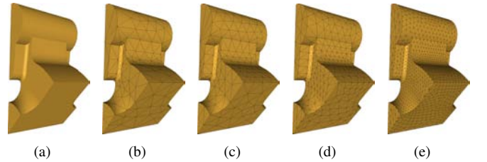
Fig. 2. (a) the CAD model of a cell for the Damped Detune Structure (DDS) for eigen-mode analysis. Only one-eighth of the geometry is shown. (b) Mesh 1 with 913 elements. (c) Mesh 2 with 1278 elements. (d) Mesh 3 with 3256 elements. (e) Mesh 4 with 19788 elements.
