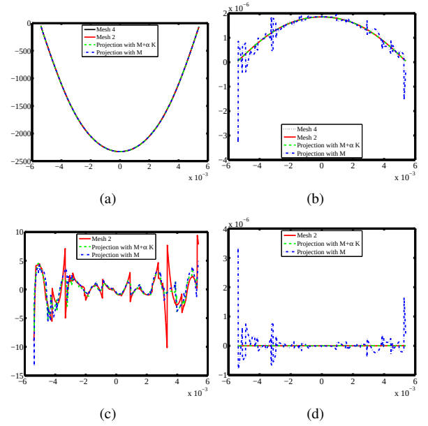
Fig. 4. (a) The electric fields computed with direct finite-element simulation using Mesh 2 and 4 and the electric fields projected from Mesh 2 to Mesh 4. (b) The magnetic fields. (c) The errors of the electric fields. (d) The errors of the magnetic fields.
