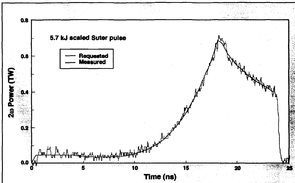
Fig. 7 An example of a shaped 2\omega pulse with total energy of 5.7 kJ and pulse length of approximately 25 ns.
